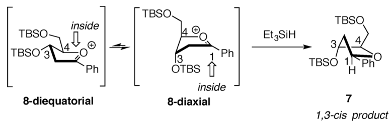
Figure 2. The stereoselectivity for 6 can be explained by the inside attack model.
