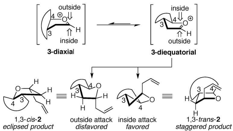
Figure 1. Reactions of fused-ring oxocarbenium ions.
