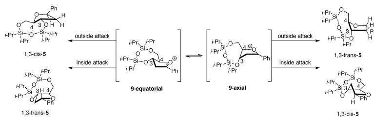
Figure 3. Possible reaction trajectories.
