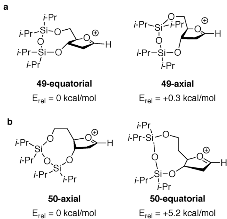
Figure 7. Calculated (B3LYP/6-31G*) enthalpies of fused-bicyclic oxocarbenium ions.
