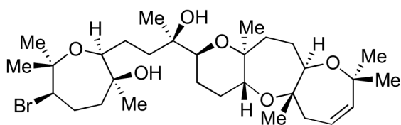
diastereomer 73
