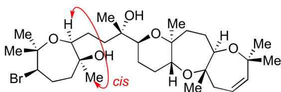
diastereomer 72
