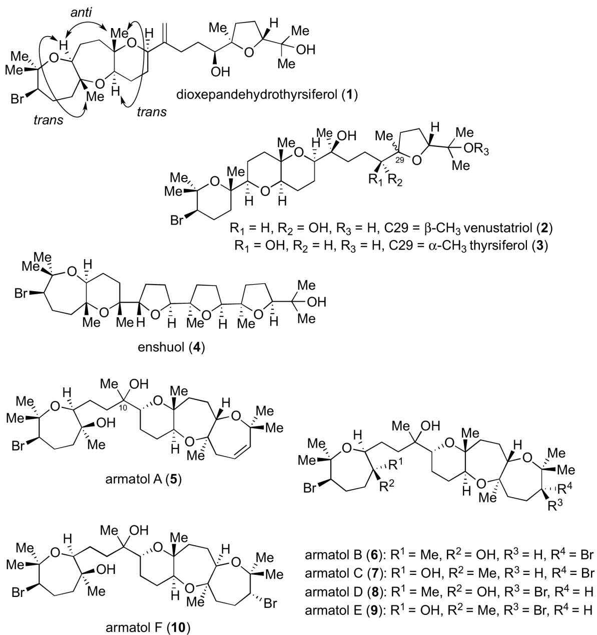
Figure 1. Representative examples of the halogenated squalene-derived terpenoid polyethers.
