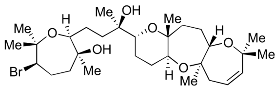
diastereomer 74
