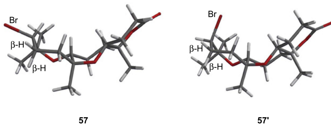
Figure 2. Computed three-dimensional structures of 57 and 57' (Spartan, HF/6-31G*).
