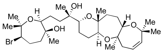
diastereomer 75
