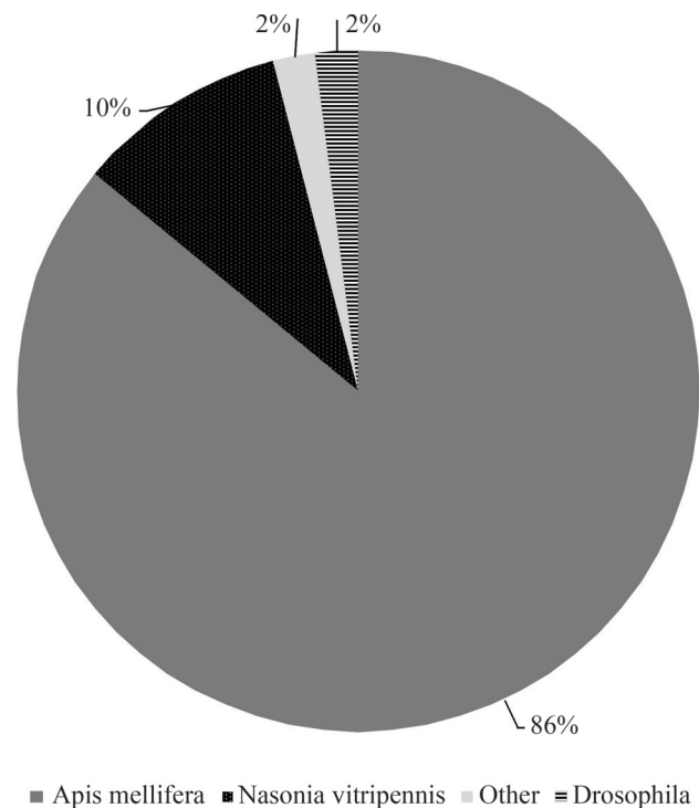
Figure 1 - Transcript distribution of the best matches of the Melipona scutellaris fat body cDNA library. The best matches were listed based on the insect species without considering E-values.
