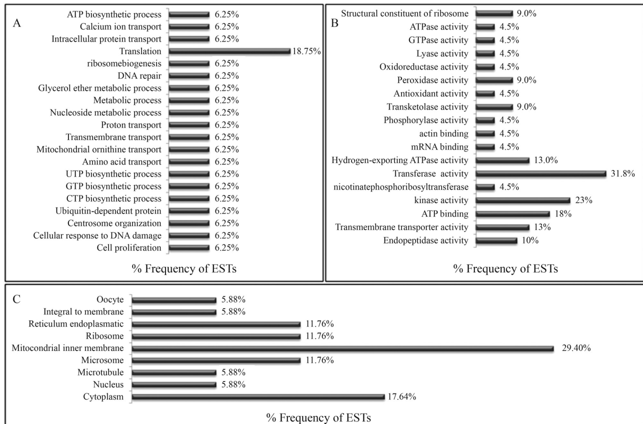
Figure 2 - Transcript distribution of Melipona scutellaris fat body cDNA library. Protein functions were assigned based on homology with Drosophila genes. (A) Biological process. (B) Molecular function. (C) Cell component.
