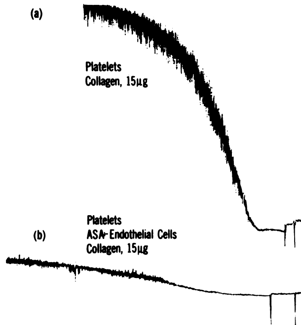
FIGURE 4 (a) Control aggregation curve with collagen (15 \mu\text{g} /cuvette) as the stimulus. (b) Effect of ASA-treated endothelial cells on the platelet response to collagen. The pattern of inhibition was similar to that observed with thrombin. \text{PGI}_2 formation was demonstrable, as shown in Table II. However, the quantity of radiolabeled 6-keto-PGF _{1\alpha} detected was lower than in the thrombin and ionophore experiments. Similar results were obtained in radioimmunoassay experiments. Total volume of test mixture was 0.5 ml.
