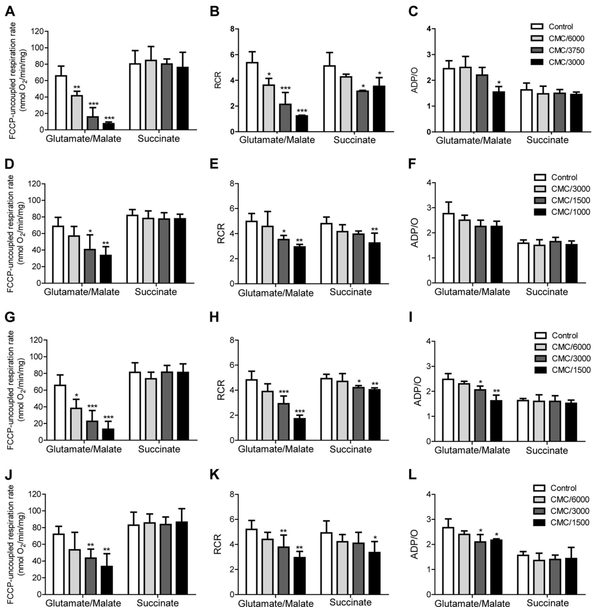
FIG 3 Effects of QAC on the respiratory activity in isolated mitochondria. The effects of C_{10} TAB (A to C), C_{12} TAB (D to F), C_{12} PB (G to I), and C_{12} BZK (J to L) on FCCP-uncoupled respiration rate (left panels), respiratory control ratio (RCR) (middle panels) and on the ADP/O ratio (right panels) were determined in isolated rat liver mitochondria after 5 min of exposure. The data are presented as means \pm the SD of at least three independent experiments. Asterisks (*, P < 0.05 ; **, P < 0.01 ; ***, P < 0.001 ) signify differences from the respective control. The CMC of each QAC is as follows: C_{10} TAB, 4.0 \times 10^{-2} M; C_{12} TAB, 3.5 \times 10^{-3} M; C_{12} PB, 3.9 \times 10^{-3} M; and C_{12} BZK, 1.7 \times 10^{-3} M.
