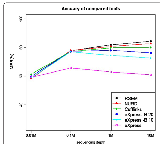
Figure 3 Comparison of estimation accuracies. Isoform expression estimation accuracies (measured by MIRR) of compared tools on the simulation data generated with genes on human chromosome 1 with different sequencing depths.
