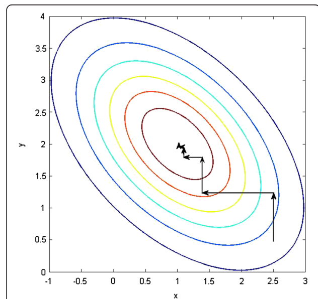
Figure 2 Illustration of 2-dimension coordinate binary search algorithm.
