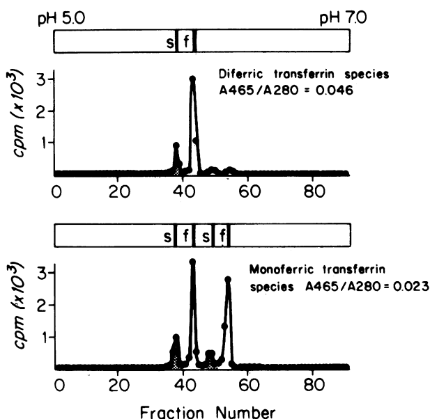
FIGURE 1 Isoelectric focusing pattern of rat plasma transferrin species. The gel was 1.4 \times 18 cm, contained 1% ampholine, pH range 5–7, and was run for 20 h at 1,000 V. The position of the visible peaks of Fe_2Tf_s , Fe_2Tf_f , the two monoferric Tf_s , and the two monoferric Tf_f are indicated. After the isoelectric focusing run the gel was cut into slices of 2 mm thickness and the radioiron content was measured. (a) Fe_2Tf_s was labeled with ^{55}Fe (shaded area) and Fe_2Tf_f was labeled with ^{59}Fe (open area). (b) Same sample as in a but after a pH step to 5.1 to produce the monoferric species. The species Fe_2Tf_f and Fe_2Tf_s were mixed in the ratio 70:30 as they occur normally in the plasma of iron-deficient rats. The radioactive counts of ^{55}Fe and ^{59}Fe per milligram transferrin were similar.
