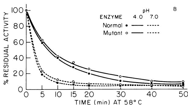
FIGURE 6 Heat denaturation curves. All samples were assayed for enzyme activity at pH 4.0. Maltose was used as substrate. (A) Acid \alpha -glucosidase in crude cultured skin fibroblast lysates from normal and adult acid \alpha -glucosidase deficiency fibroblasts. The activity at zero time (100% activity) was 223 and 74 \mu g glucose released per milligram protein per hour for the normal and the deficient cells, respectively. The normal fibroblasts were harvested at early confluency, whereas the mutant cells were harvested at late confluency to increase the specific activity. Cells were lysed and heated in 0.1 M (in reference to phosphate) citrate-phosphate buffer, pH 4.0. (B) Purified acid \alpha -glucosidase from normal and adult acid \alpha -glucosidase deficiency fibroblasts heated at pH 4.0 and 7.0 in 0.1 M (in reference to phosphate) citrate-phosphate buffer. The enzyme preparations from the normal and deficient cells contained 74 and 40 U acid \alpha -glucosidase, respectively. Both preparations contained 0.8 mg bovine albumin per milliliter added to stabilize the enzyme. Conc, concentration.
