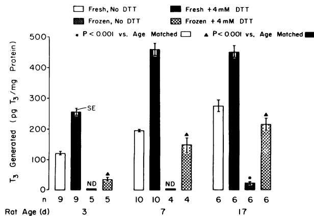
FIGURE 1 Effect of DTT on in vitro H- \text{T}_3 in neonatal homogenates frozen for 6 mo at -20^{\circ}\text{C} . Homogenates were incubated with 0.5\ \mu\text{g} \text{T}_4/1\ \text{ml} homogenate at 37^{\circ}\text{C} for 15 min. n denotes the number of rats in each group, or in the case of neonatal rats < 12\ \text{d} of age, the number of homogenate pools in each group. Significance calculated by the Student's t test.
