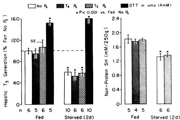
FIGURE 7 Effect of starvation and T 4 (1.5 μg/100 g per d, i.p. × 10 d) or T 3 (0.5 μg/100 g per d, i.p. × 10 d) administration on hepatic NPSH groups and DTT stimulation of H-T 3 . For other details, see Fig. 1.
