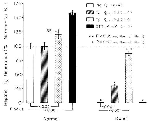
FIGURE 5 Effect of T 4 (1.5 μg/100 g per d, s.c.) or T 3 (0.5 μg/100 g per d, s.c.) administration and in vitro addition of DTT on H-T 3 in the normal and hypopituitary, hypothyroid dwarf mouse. For other details, see Fig. 1.
