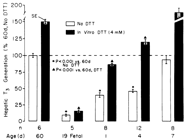
FIGURE 6 Effect of age on DTT stimulation of in vitro H-T 3 in the rat. For other details, see Fig. 1.
