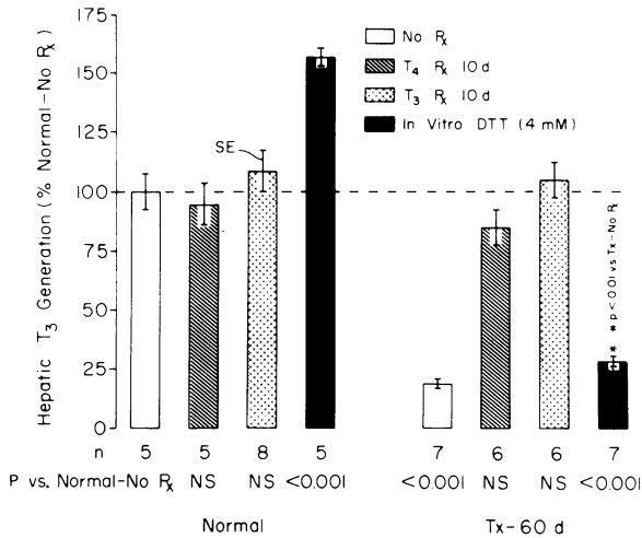
FIGURE 3 Effect of thyroidectomy (Tx) and T 4 (1.5 μg/100 g per d, i.p.) or T 3 (0.5 μg/100 g per d, i.p.) treatment and in vitro addition of DTT on H-T 3 in the rat. For other details, see Fig. 1.
