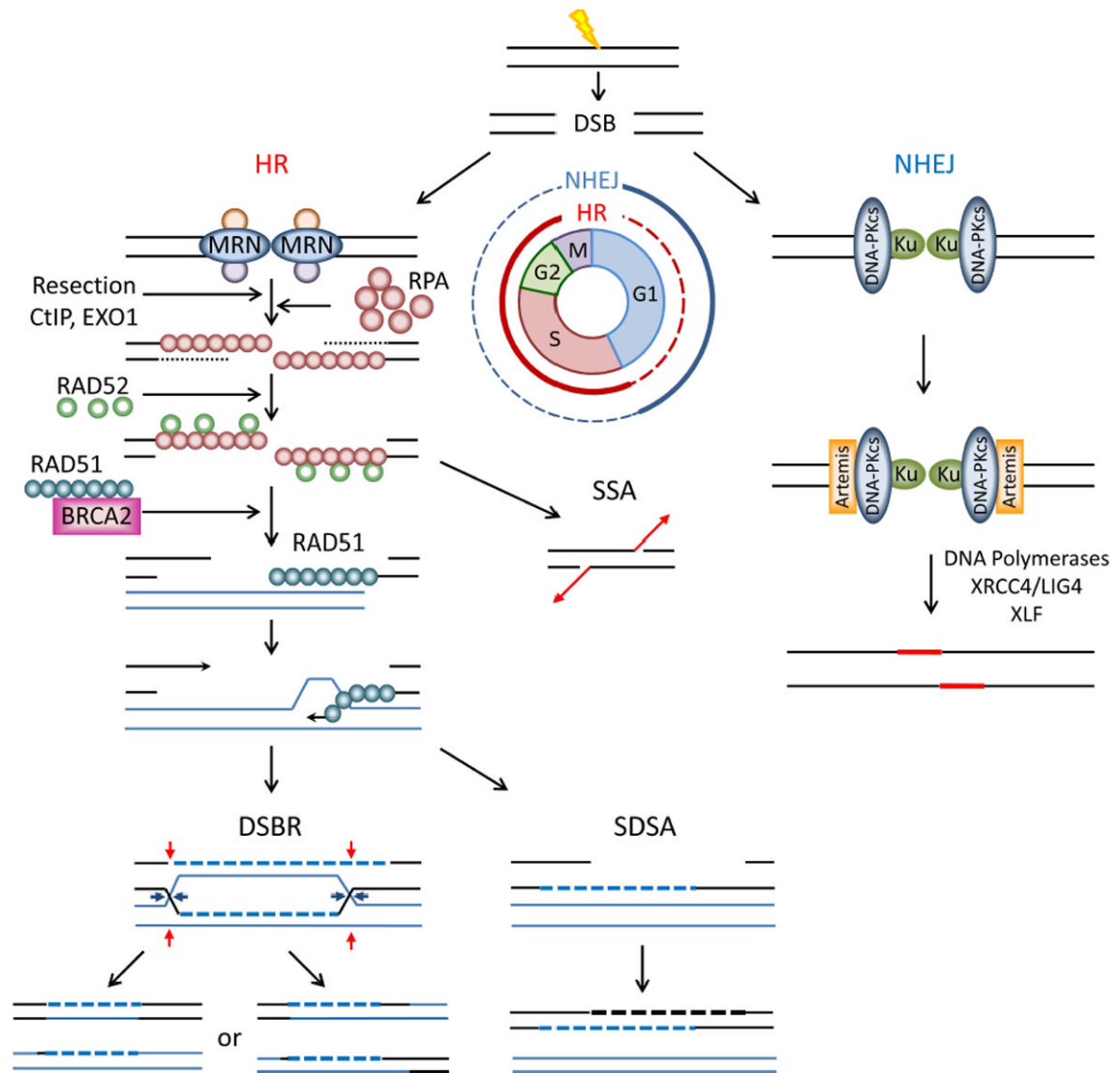
Figure 4. Recombination pathways
