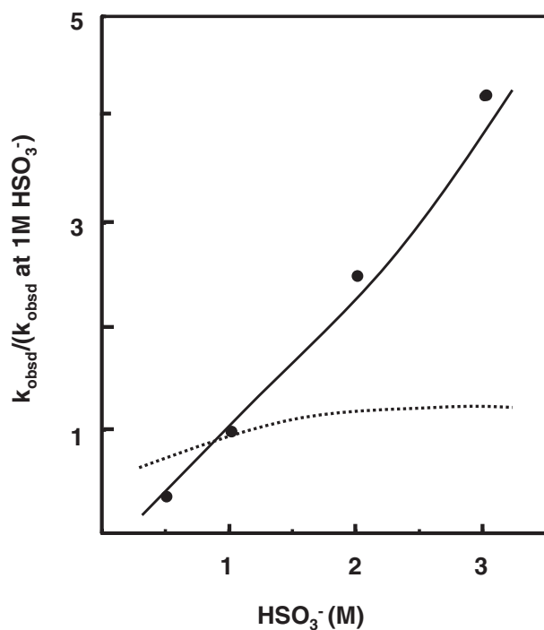
Fig. 8. Relationship between bisulfite concentration and rate of deamination of cytidine 5'-phosphate at pH 5.0 and 37 °C. The dotted line represents rates with no participation of bisulfite in hydrolyzing [C-SO 3 - ], and the solid line those predicted in case of participation of bisulfite in the process of hydrolysis.
