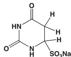
Fig. 4. Uracil-bisulfite adduct.
