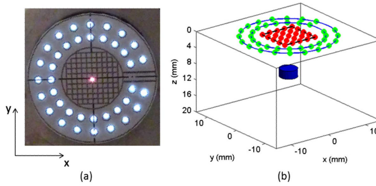
Fig. 2. (Color online) (a) Photograph of the end view of the imaging probe with the grid paper attached and with one laser scanning position (red center) shown, (b) arrangement of the sources (inner red dots) and detectors (green dots on outer rings) for FMT and one target (blue below).
