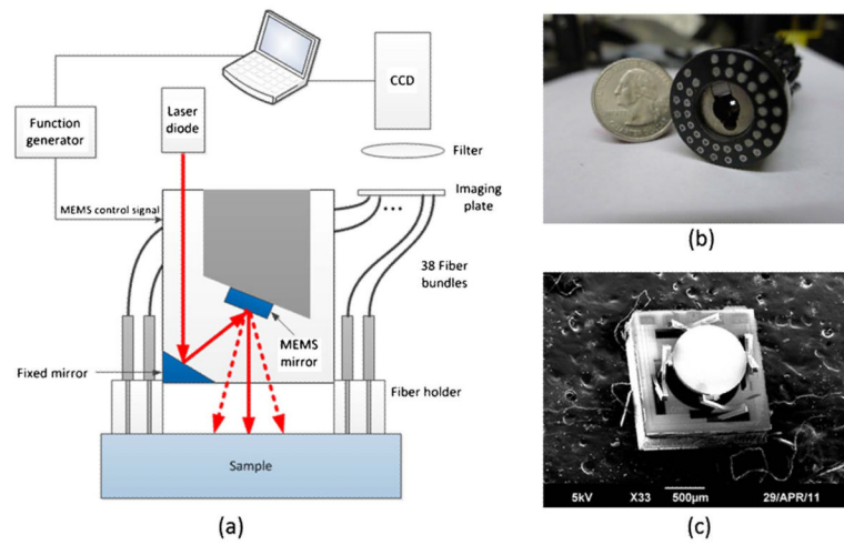
Fig. 1. (Color online) (a) Schematic of the MEMS-based FMT system, (b) photograph of the imaging probe, and (c) scanning electron microscopic (SEM) image of the MEMS mirror.
