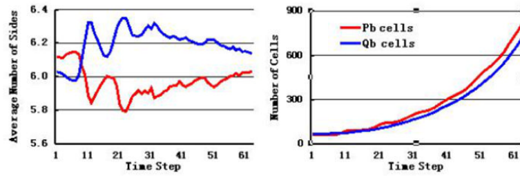
Fig. 3. Simulation results of shapes and number of cells located on the boundary between quiescent cells and proliferating cells. Left, average number of sides of BP cells decreases (red), and the average number of sides of BQ cells increases (blue). Right, the number of BP cells increases beyond that of the BQ cells during the process of growth and division.
