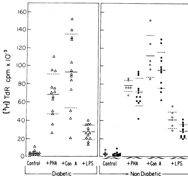
FIGURE 1 Mitogenic response of spleen cells to PHA (1 \mu\text{g/ml} ), Con A (2.5 \mu\text{g/ml} ), and E. coli LPS, 100 \mu\text{g/ml} ) from 3-month-old diabetic ( db+/db+ , \Delta ) and nondiabetic ( db+/m+ , \bullet , and m+/m+ , \circ ) mice. 0.5 \times 10^6 spleen cells from individual mice were cultured in triplicate in the presence of mitogen for 64 h. The results represent the mean \pm 1 SD.
