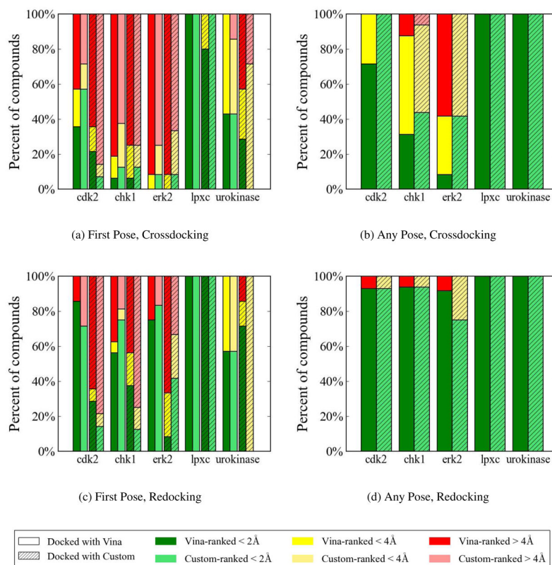
Figure 5. The docking results for all protein targets using Vina and our custom scoring function. In (a) and (c) there are four bars for each target, one for each dock-rank method. For each target the bars are, in order left to right: Vina-Vina, Vina-custom, custom-Vina, and custom-custom. (a) The RMSD for the top ranked (by predicted affinity) pose of each compound when crossdocking using each dock-rank method. (b) The RMSD of the lowest RMSD pose of all returned poses for a compound when crossdocking. (c) and (d) The same as (a) and (b) but for redocking.
