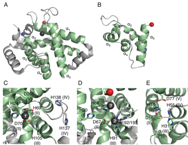
Figure 9 The structures of Cas protein HD domains
