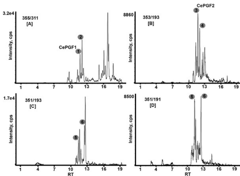
Figure 3. MRM analyses of wild-type extracts. F1 class PGs are detected with mass transition m/z 355/311 [A]. Notice that several hydrophobic compounds (RT > 14 min), which are unlikely to be PGs, are also detected with this transition. F2 class PGs are detected with mass transition m/z 353/193 [B]. F3 class PGs are detected with either mass transition m/z 351/193 [C] or m/z 351/191 [D]. Notice that the extracts contain multiple PG isomers of each class. Numbers correspond to PGs shown in Table 2. The concentration of CePGF2 is 1.8 ng/ml. RT, retention time; cps, counts/sec.
