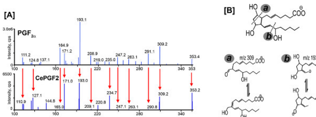
Figure 4. Collision-induced decomposition of chemically synthesized PGF 2α and CePGF2. Arrows in panel [A] indicate product or fragmentation ions shared between PGF 2α and CePGF2 (RT=11.8). The product ions at m/z 309 and m/z 193 are generated from indicated cleavage sites (highlighted a and b ), correspond to the structures shown, and are characteristic of F-series PGs [B]. Cps, counts/sec. Click here to view larger figure.
