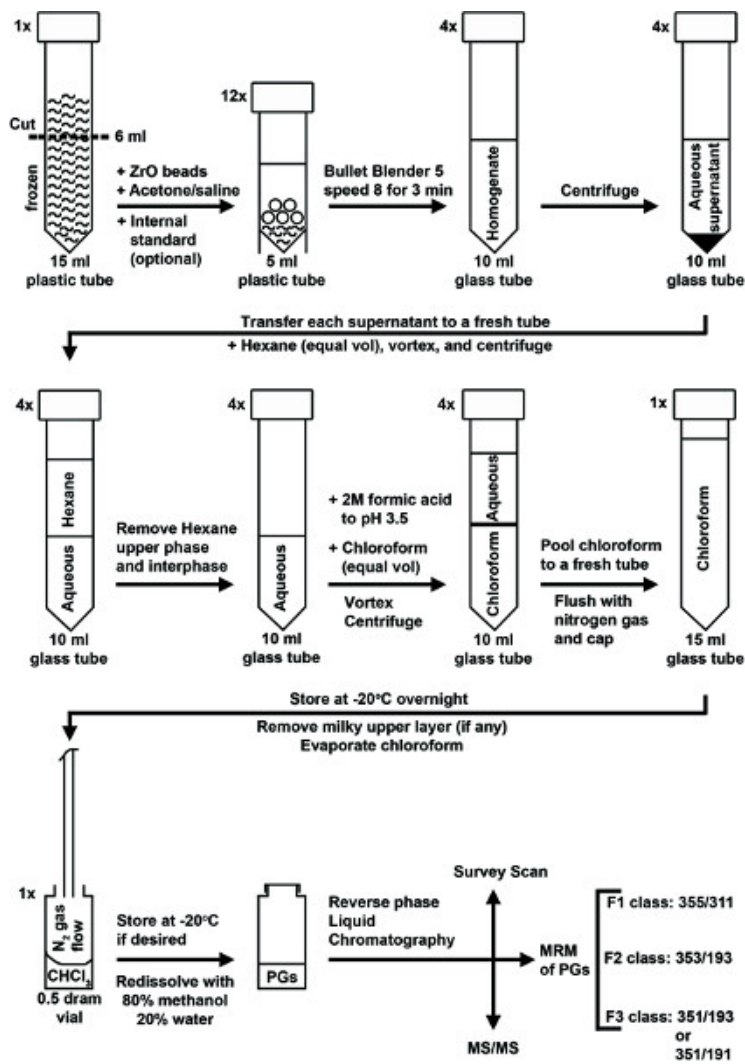
Figure 1. Schematic diagram of C. elegans PGs extraction and LC-MS analyses. Note that acetone/saline and chloroform both have 0.005% BHT to minimize lipid oxidation. Refer to the text for more details. Click here to view larger figure.
