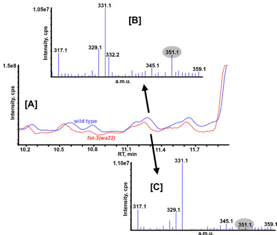
Figure 2. Survey scans of m/z 315-360 of wild-type and fat-3(wa22) mutant extracts. Liquid chromatography retention time (RT) is shown in panel [A]. Extracted ions at RT = 11.3 are shown for wild-type [B] and fat-3(wa22) [C] extracts. An F3 class PG with mass m/z 351 is highlighted. Cps, counts/sec; a.m.u., atomic mass unit.
