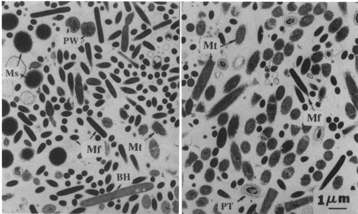
FIG. 14. Transmission electron micrographs of syntrophic biomethanation granules. Mf, Methanobacterium formicum -like rods; Mt, Methanotrux -like rods; Ms, Methanosarcina mazei -like cocci; BH, sporeforming Syntrophospora bryantii -like rods; PT, sporeforming propionate degrader; PW, nonsporeforming propionate degrader. Note that the syntrophiles are surrounded by H_2 - and formate-consuming methanogens. Reprinted from reference 478 with permission.
