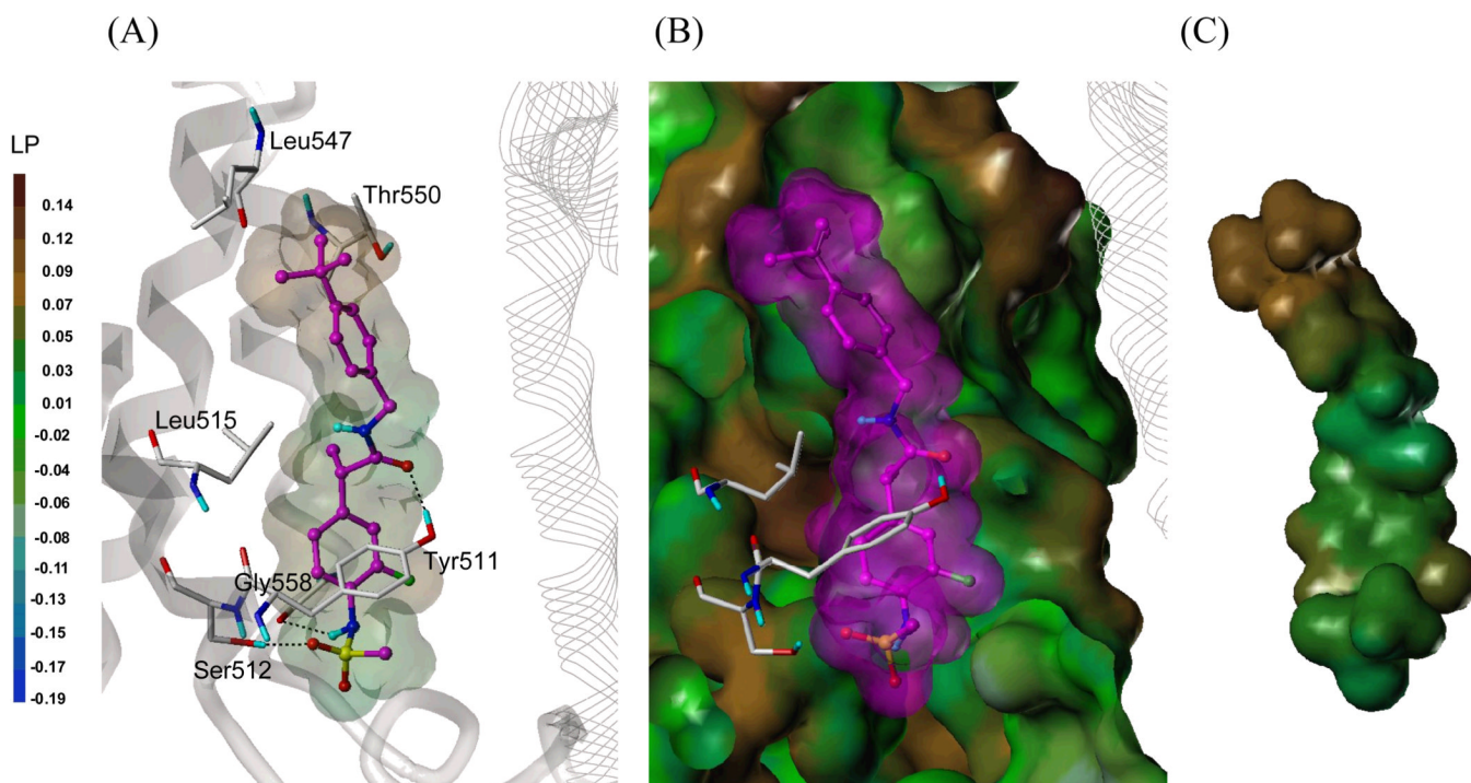
Figure 2. Predicted binding mode of 54S in hTRPV1 homology model with surface representations
