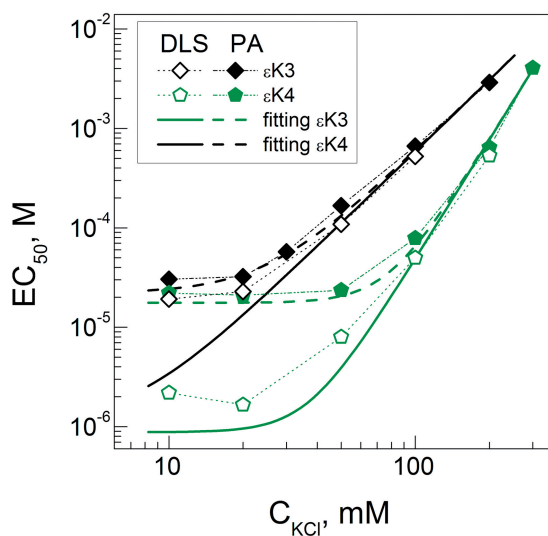
Figure 9. Comparison of the experimental dependencies (points with thin lines) with prediction based on Equation (3) (shown as smooth thick lines) for data on DNA condensation by the \epsilon -oligolysines \epsilon K3 and \epsilon K4. DLS and PA data are shown respectively as hollow and solid points. The parameters of Equation (3) are the same as in Figure 8A. See text and Supplementary Figure 4S and Table 4S) for more detail.
