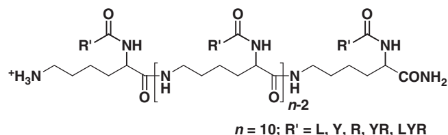
Figure 1. Chemical structures of linear \epsilon -oligolysines and \alpha -substituted derivatives of \epsilon K10. (L, Y and R represent amino-acid residue leucine, tyrosine and arginine, respectively).
