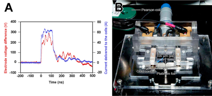
Figure 1. Microscope stage-mounted slide holder with contact electrodes and waveform. A. Oscilloscope trace of the 100 ns long voltage (red) and current (blue) pulse applied to the cells using the chamber on the right. B. Chamber that mounts on the microscope stage to apply the pulse to the cells in the 100 \mu\text{m} -wide gap between two pieces of Pt foil.
