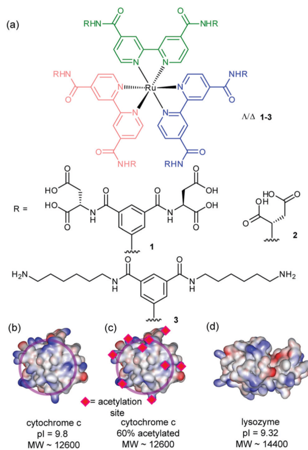
Fig. 1. Structures of receptors and proteins (together with relevant properties) described in this work (a) highly functionalized ruthenium tris-bipyridine receptors 1–3 (b) cytochrome c (PDB ID 1HRC), 31 (c) 60% acetylated cytochrome c (d) lysozyme (PDB ID 2LYM). 32
