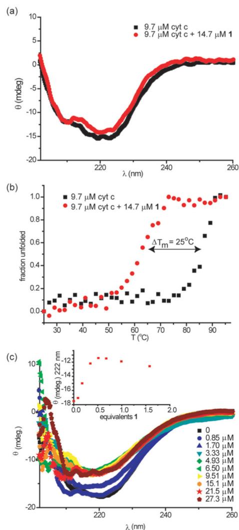
Fig. 2. Perturbations to secondary structure of cyt c in the presence of 1 (5 mM sodium phosphate, pH 7.4), (a) circular dichroism spectra of cyt c (9.7 μM) in the absence and presence of 1 (14.7 μM) at 25 °C, (b) thermal melting profiles of samples from (a) and (c) circular dichroism spectrum of 9.6 μM cyt c upon titration with 1 at 70 °C (inset: illustrates titration curve).
