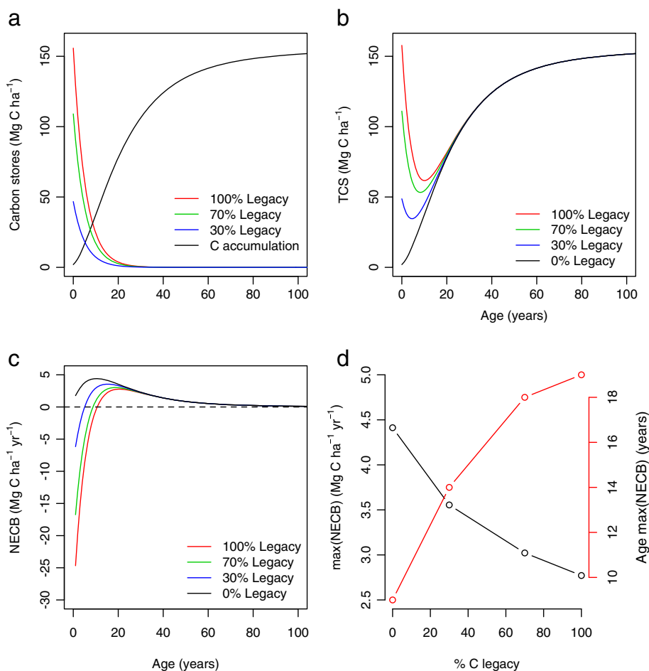
Figure 4 Effects of carbon legacies on total carbon accumulation and net ecosystem carbon balance (NECB). a ) Temporal behavior of legacy carbon (colored lines) and new carbon accumulation (black line). b ) Total carbon stocks (TCS) under different assumptions of carbon legacies. c ) Net ecosystem carbon balance (NECB) under different assumptions of C legacies. d ) Effects of C legacies on the maximum accumulation rates (max(NECB)), and the age at which this rate is reached (Age max(NECB)). % C legacy represents the percentage of C left in situ to decompose from the total carbon mass (TM) present in undisturbed forests. Decomposition of C legacies according to decomposition rates reported by [24].
