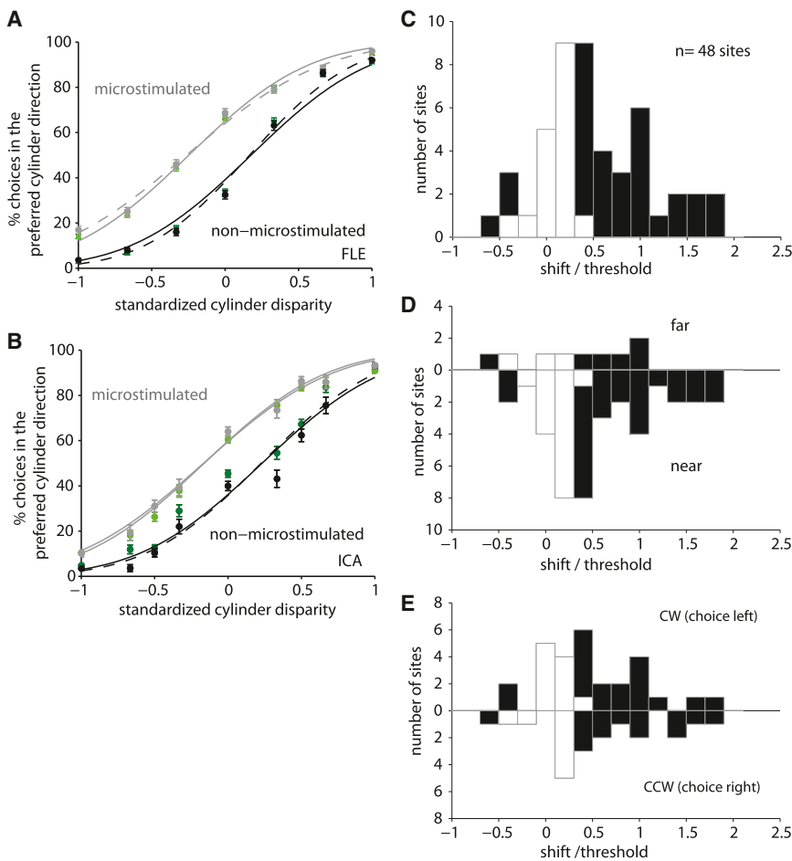
Figure 3. Summary of the Microstimulation Effect (A) This figure illustrates the shifts when we fitted the standardized psychophysical data pooled across microstimulation sites in monkey FLE. The range of cylinder disparities was standardized for all 20 microstimulation sites, such that the largest disparities at each site were set equal to -1 and 1 . Data were averaged across sites. The proportion of choices in the preferred direction was plotted against the standardized cylinder disparity, and pairs of cumulative Gaussians were fitted. Data from all sites are shown in green; data for sites with a significant shift are shown in black and gray. For the significant stimulation sites, one pair of fits, for microstimulated (in gray) and nonmicrostimulated trials (in black), was only allowed to differ in their horizontal offset (solid line); the other pair in offset and slope ( 1/SD ) of the fitted curve (dashed line). For FLE, the pooled shift measured +0.42 and the SD (which is a measure of psychometric threshold) was 0.64 . This yields a ratio of shift/SD of 0.66 , equivalent to almost two thirds of threshold. The pooled data for all microstimulation sites (green) shows an almost identical pattern (shift/SD = 0.62 ). The difference is small because most sites showed a significant shift and there were two significant shifts in the nonpreferred direction. Error bars depict the SEM. (B) For monkey ICA, response data were standardized and pooled for microstimulation sites with significant shifts (in black and gray) and across all sites (in green), as in (A). The pooled shift for significant microstimulation sites measured +0.39 and the SD 0.66 . The shift is equivalent to about two thirds of threshold (SD), with a ratio of shift/SD of 0.59 (for all sites shift/SD = 0.36 ). (C) The distribution of normalized microstimulation shifts across all 48 sites from both monkeys is shown. The majority of significant horizontal
