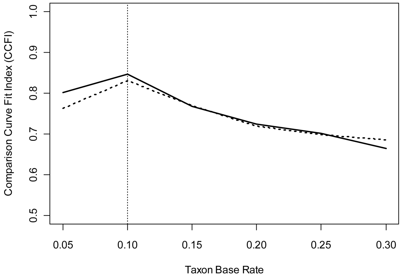
Figure 6. CCFI values for taxometric analyses performed using different taxon base rates. The dotted line shows results for L-Mode, the solid line shows the averaged results for MAMBAC, MAXEIG, and L-Mode. The vertical line highlights the actual taxon base rate ( P = .10 ) for these data.
