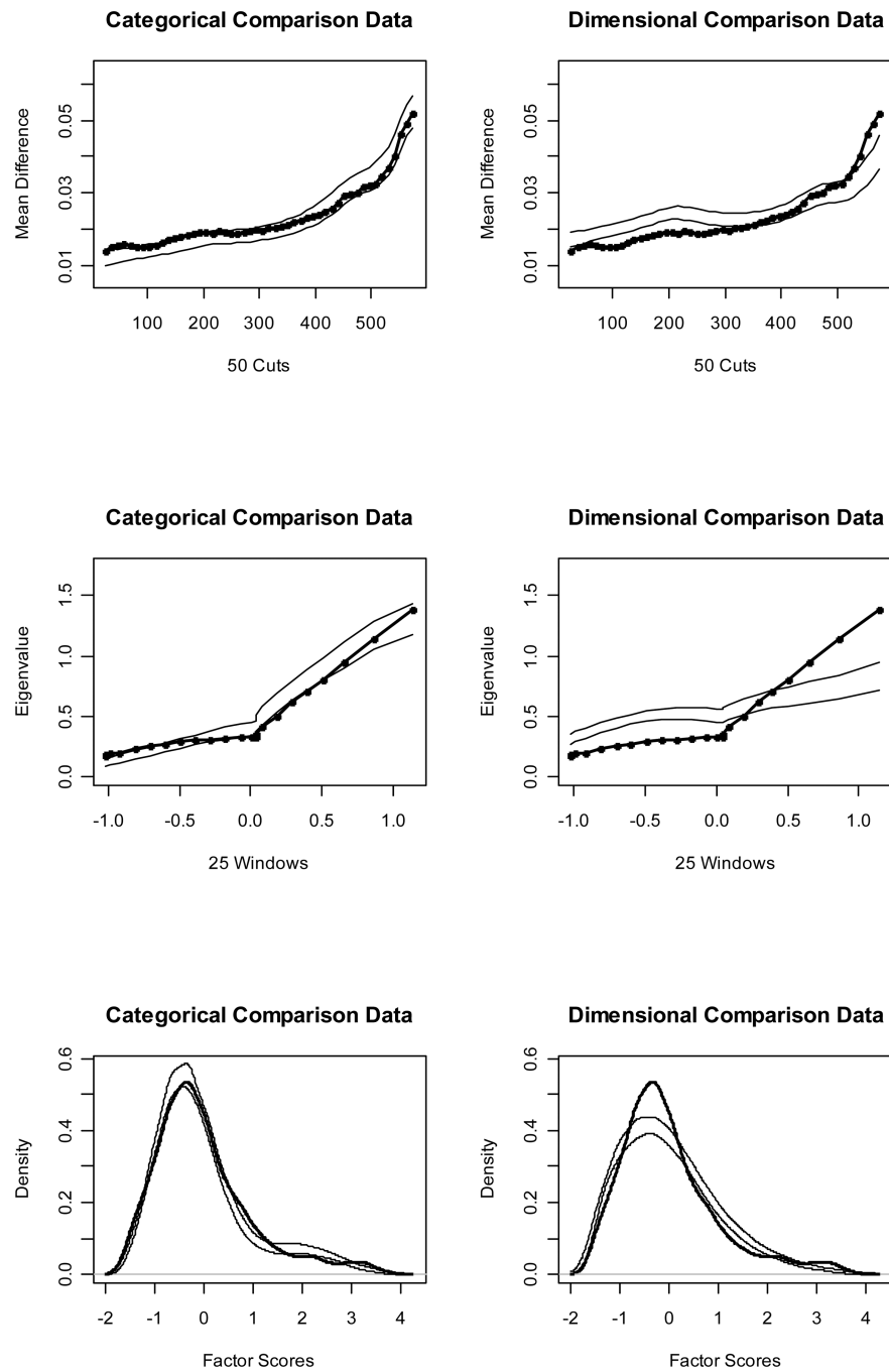
Figure 3. Results for MAMBAC (top), MAXEIG (middle), and L-Mode bottom) analyses of the representative categorical (RC) data set. Dark lines show the results for the RC data set, and lighter lines show the results for parallel analyses of comparison data; the lines contain a band that spans \pm 1 SD from the M at each data point on the curve.
