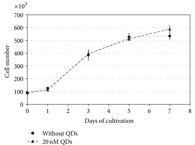
FIGURE 8: Growth curve of QD labeled and unlabeled stem cell populations during 7 days of cultivation. Cells were counted on days 1, 3, 5, and 7. Mean cell count was calculated from three experiments.
