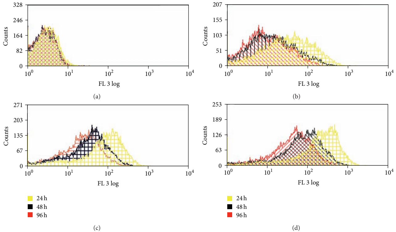
FIGURE 3: FACS analysis of QDs cell load over cultivation time. The fluorescence per cell was analysed after 24 h, 48 h, and 96 h. (a) Control cells without QDs, (b) cells labeled with 5 nM QDs, (c) cells labeled with 10 nM QDs, and (d) cells labelled with 20 nM QDs.
