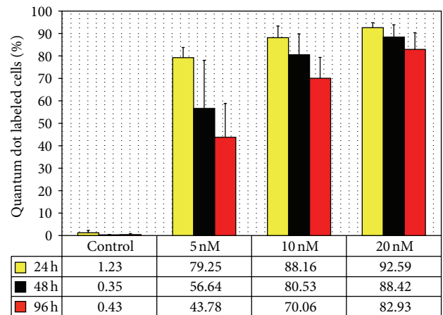
FIGURE 4: Quantitative analysis of QD labeled cells measured by FACS analysis. The amount of QD labeled cells was estimated for three label concentrations (5 nM, 10 nM, and 20 nM) and for three time points (24 h, 48 h, and 96 h) ( n = 2 ). Total count 10.000 cells.
