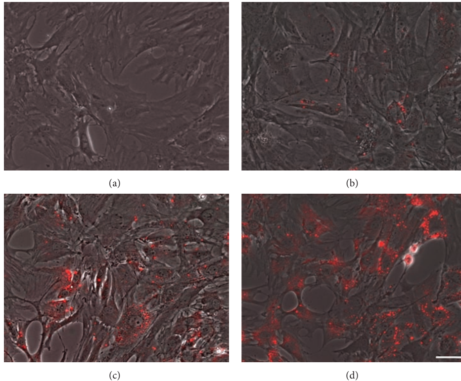
FIGURE 1: Fluorescence intensity and distribution of QD treated living stem cells 24 h after labeling. (a) Control without QDs, (b) 5 nM QDs, (c) 10 nM QDs, and (d) 20 nM QDs. Scale bar represents 50 \mu\text{m} .
