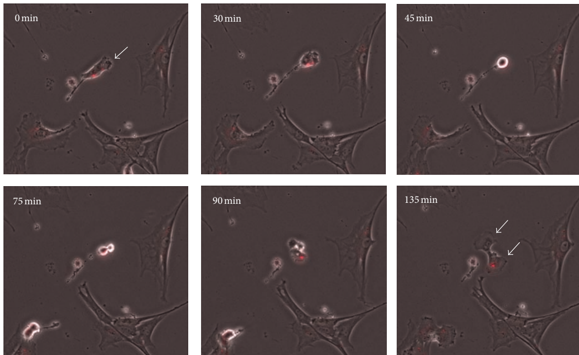
FIGURE 6: Time-lapse study showing unequal passing on of QDs during cell division (see arrows). Selected microscopy images acquired during cultivation of labeled cells show a time period of 135 min. Overlay images were created from the fluorescent and the phase contrast image.
