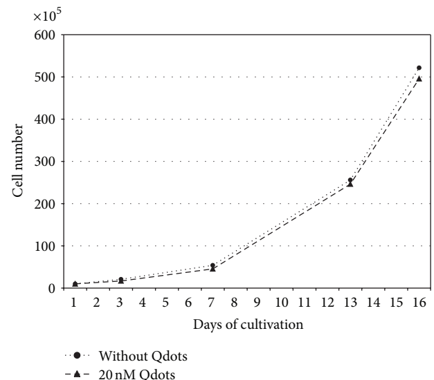
FIGURE 9: Long-term proliferation of a QD labeled and an unlabeled stem cell population during subcultivation within a period of 16 days. The cells were passaged and counted on days 3, 7, 13, and 16. Curve was calculated from one experiment.
