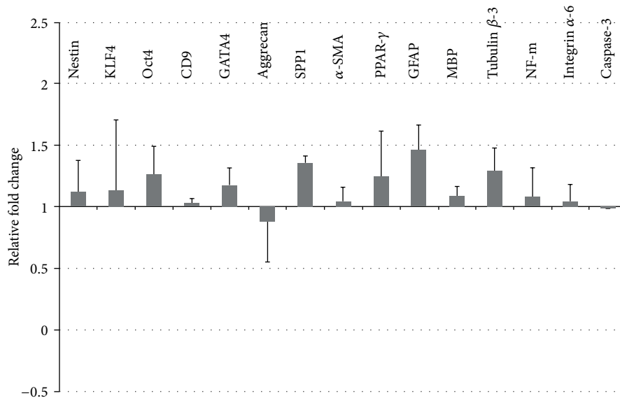
FIGURE 10: The transcriptional activity of QD labeled stem cells was analyzed by quantitative PCR and set in relation to untreated control approaches (representing the value “1”). Changes in gene expression are displayed as upregulation ( >1 ) and downregulation ( <1 ). Standard deviations were calculated from two experiments. Transcripts related to stem cells (Nestin, KLF4, Oct4, CD9), endodermal cells (GATA4), mesodermal cells (Aggrecan, SPP1, \alpha -SMA, PPAR- \gamma ), and ectodermal cells (GFAP, Tubulin \beta -3, NF) were analyzed. Also the mRNA expression level of the surface protein Integrin alpha-6 and the apoptosis marker caspase-3 was estimated.
