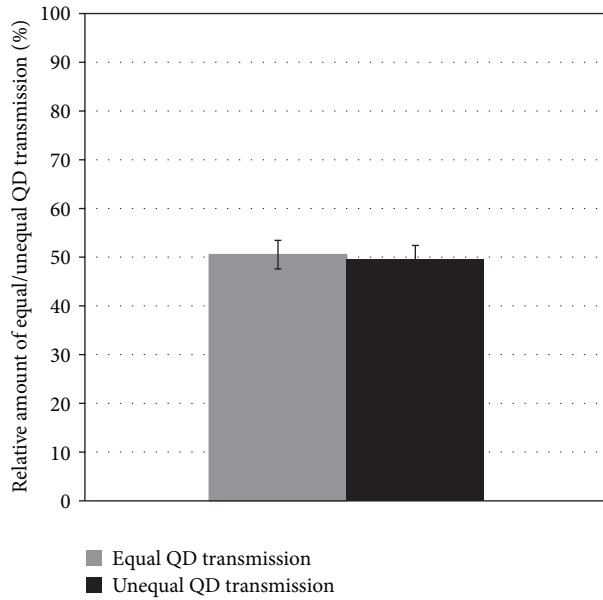
FIGURE 7: Distribution of equal and unequal cell divisions in QD labeled cell populations. The relative amount of cell divisions with equally and unequally transferred QDs was quantified by analyzing time lapse picture series of four experiments. In total, 242 cell divisions were prorated to the equal and unequal way of QD transmission.
