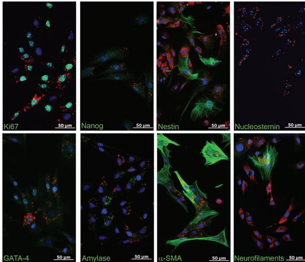
FIGURE 11: Immunocytochemical localization of stem cell and lineage specific proteins (green) in QD labeled (red) stem cells. QD labeled cells stained positive for nuclear (Ki67, Nanog, Nucleostemin, GATA-4), secretory (Amylase), and filamentous proteins (Nestin, \alpha -SMA, Neurofilaments) indicating spontaneous in vitro differentiation. Nuclei were stained with DAPI (blue).
