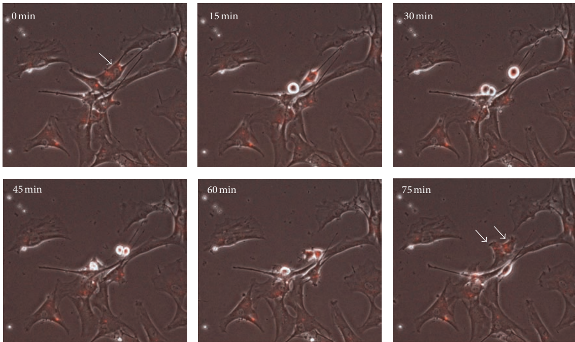
FIGURE 5: Time-lapse study showing equal passing on of QDs during cell division (see arrows). Selected microscopy images acquired during cultivation of labeled cells show a time period of 75 min. Overlay images were created from the fluorescent and the phase contrast image.
