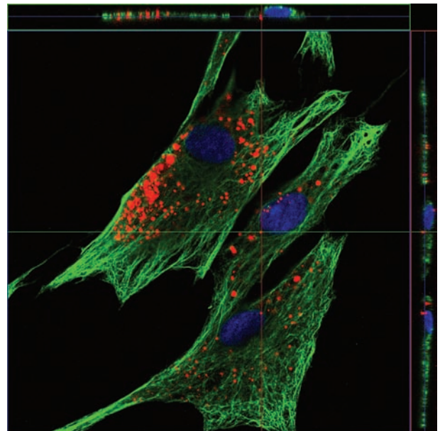
FIGURE 2: Spatial distribution of QDs (red) within the cells. Confocal image of labeled PSCs immunostained for Vimentin (green). Nuclei were stained with DAPI (blue).
