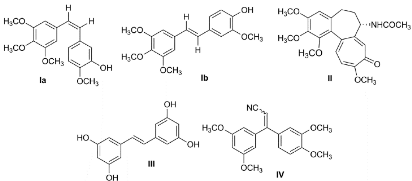
Fig 1. Chemical structures of naturally occurring antitubulin agents and their related analogs
