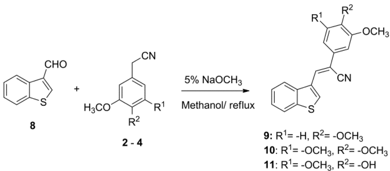
Scheme 2. Synthesis of Z -benzo[ b ]thiophene-3-yl acrylonitriles
