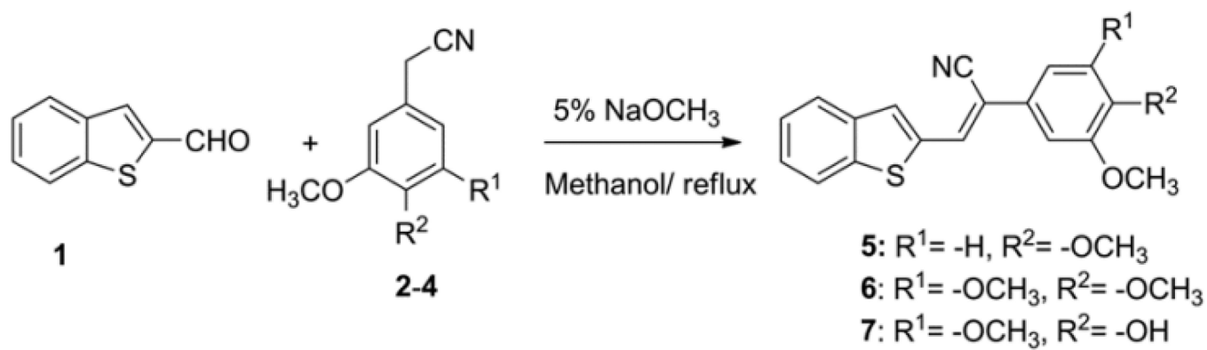
Scheme 1. Synthesis of ( Z )-benzo[ b ]thiophene-2-yl acrylonitriles
