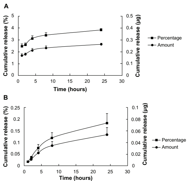
Figure 3 In vitro release study of saquinavir (SQV) from 1% hydroxyethylcellulose (HEC) gel loaded with SQV-encapsulated nanoparticles (A). Release study conducted in microcentrifuge tubes (B) release study conducted in Franz cells. The results show cumulative amounts (filled circles) and cumulative percentage released (filled squares) at 37°C in phosphate-buffered saline (pH 4.6). Values represent means ± standard deviation; n = 3.
