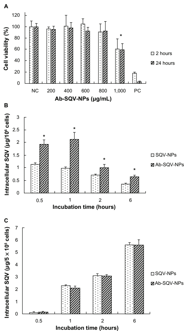
Figure 5 (A) Cytotoxicity of antibody-conjugated saquinavir-encapsulated nanoparticles (Ab-SQV-NPs) in Sup-T1 cells. The data shown represent means ± standard deviation; n = 4. (B) Intracellular accumulation of SQV in Sup-T1 cells, and (C) intracellular accumulation of SQV in VK2/E6E7 cells; values represent means ± standard deviation; n = 5.
