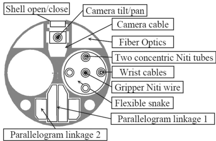
Fig. 15. Cross section of the IREP central stem.
