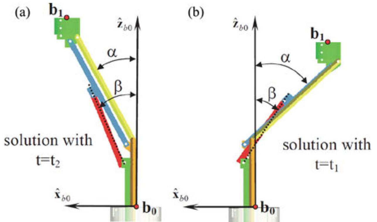
Fig. 3. Direct kinematics solutions that correspond to Table III.
