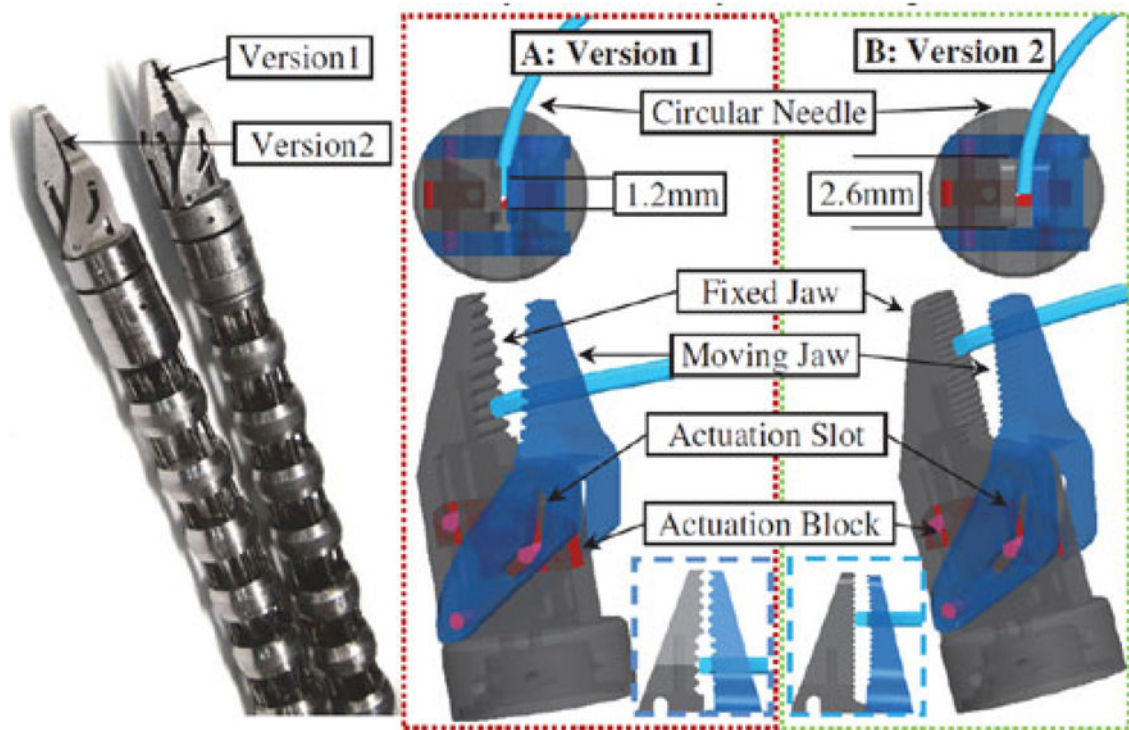
Fig. 12. Iterations of the distal wrist-gripper assembly.
