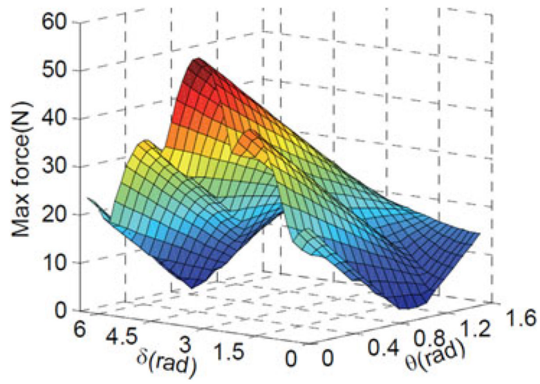
Fig. 7. Estimation of the required snake segment actuation force.
