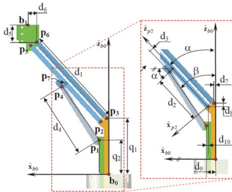
Fig. 2. Dimensions and nomenclature used for forward kinematics.
