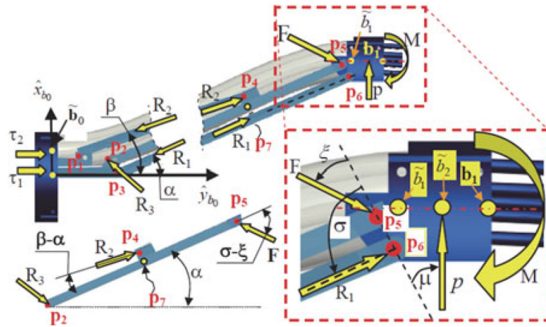
Fig. 10. Free body diagram of the forces acting on the moving base ring of the parallelogram linkage.
