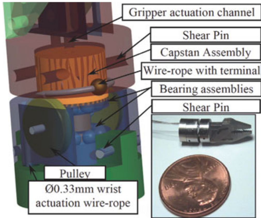
Fig. 13. Prototype of wrist and gripper.
