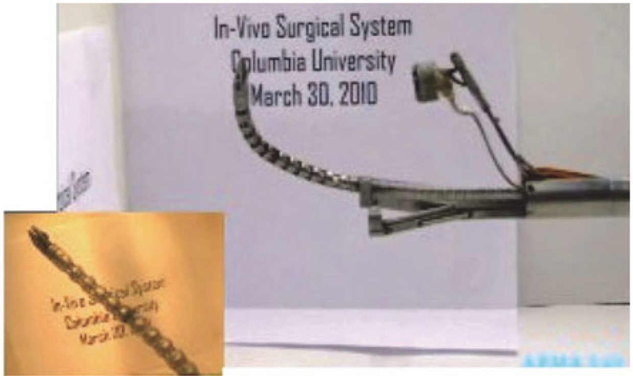
Fig. 20. One IREP arm with the camera mechanism deployed. The inset shows the view from the IREP camera.
