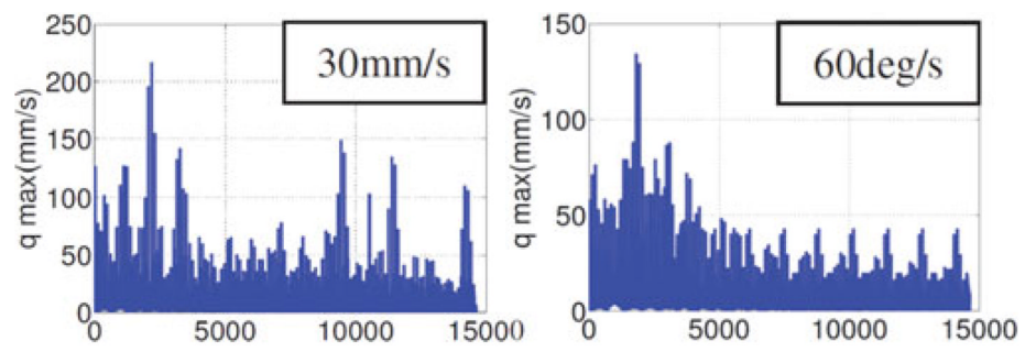
Fig. 6. Maximal required joint speed for a two-stage continuum robot.
