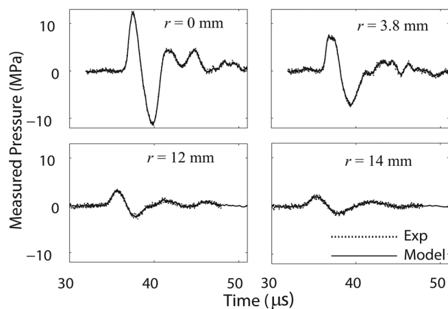
FIG. 4. Selected radial scan averaged waveforms collected from the measurements in a plane 5 mm from the short standoff, along with simulation fit from model. Radial scan had a total length of 14 mm and waveforms along the way were used as a boundary condition for the model.
