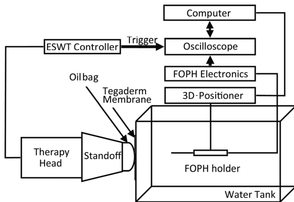
FIG. 2. Illustration of experimental setup. The therapy head can be either ballistic (no standoff used) or electromagnetic (as shown). Coupling of the treatment head to the water was facilitated by a Tegaderm window and coupling gel.
