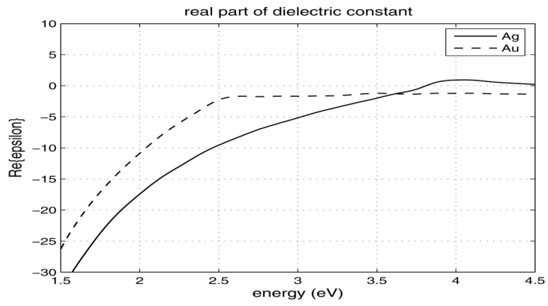
Fig. 1. Real part of dielectric constant (from [7]).
