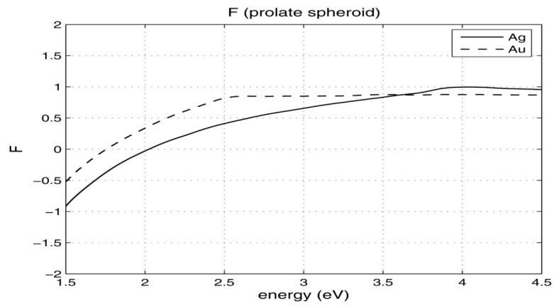
Fig. 2. Plot of the function F(\omega) given by Eq. (14) for a prolate spheroid.
