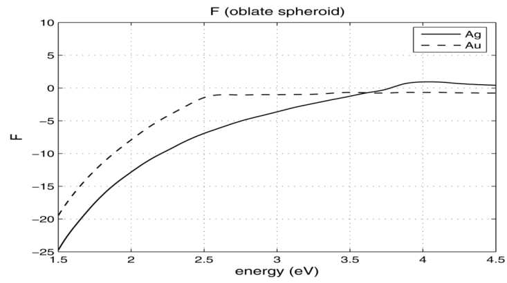
Fig. 3. Plot of the function F(\omega) given by Eq. (14) for an oblate spheroid.
