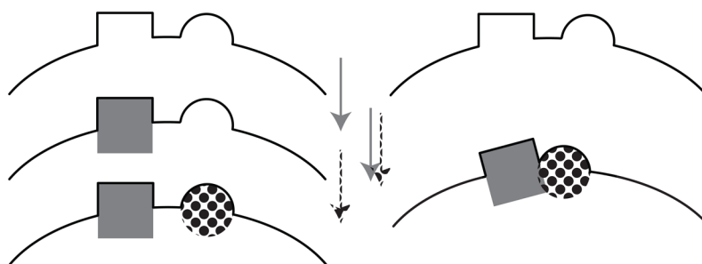
Figure 1. Multiple ligand docking. Black curve represents a protein interface. Square and circle represent two ligands. Often multiple ligands, cofactors, water molecules, and ions interact with a protein in a synergistic manner to produce the resultant interface structure. Using ligand docking software to dock each of these components separately (Left) may fail to capture protein induced-fit effects. Simultaneous docking of multiple ligands (Right) with backbone and side-chain flexibility improves modeling of interfaces – especially those with induced-fit effects.
