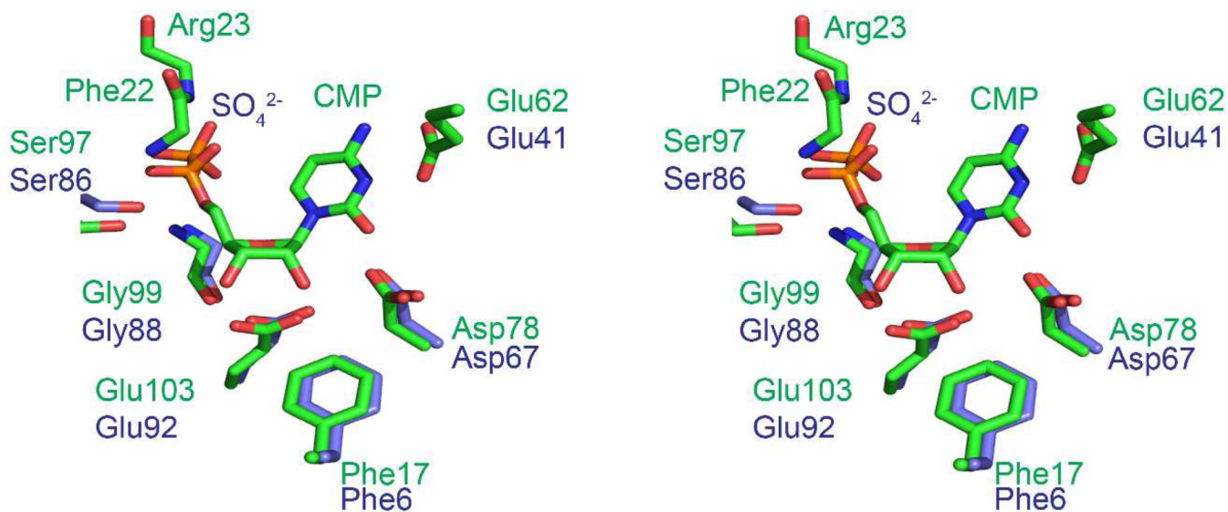
Figure 4. BcmB/PO 4 and MilB/CMP active site comparison. A stereoview of BcmB/PO 4 and MilB/CMP active sites superimposed. The active site residues of BcmB and MilB display a conserved architecture. Glu41 is disordered in the BcmB structure but conserved in sequence with MilB Glu62.
