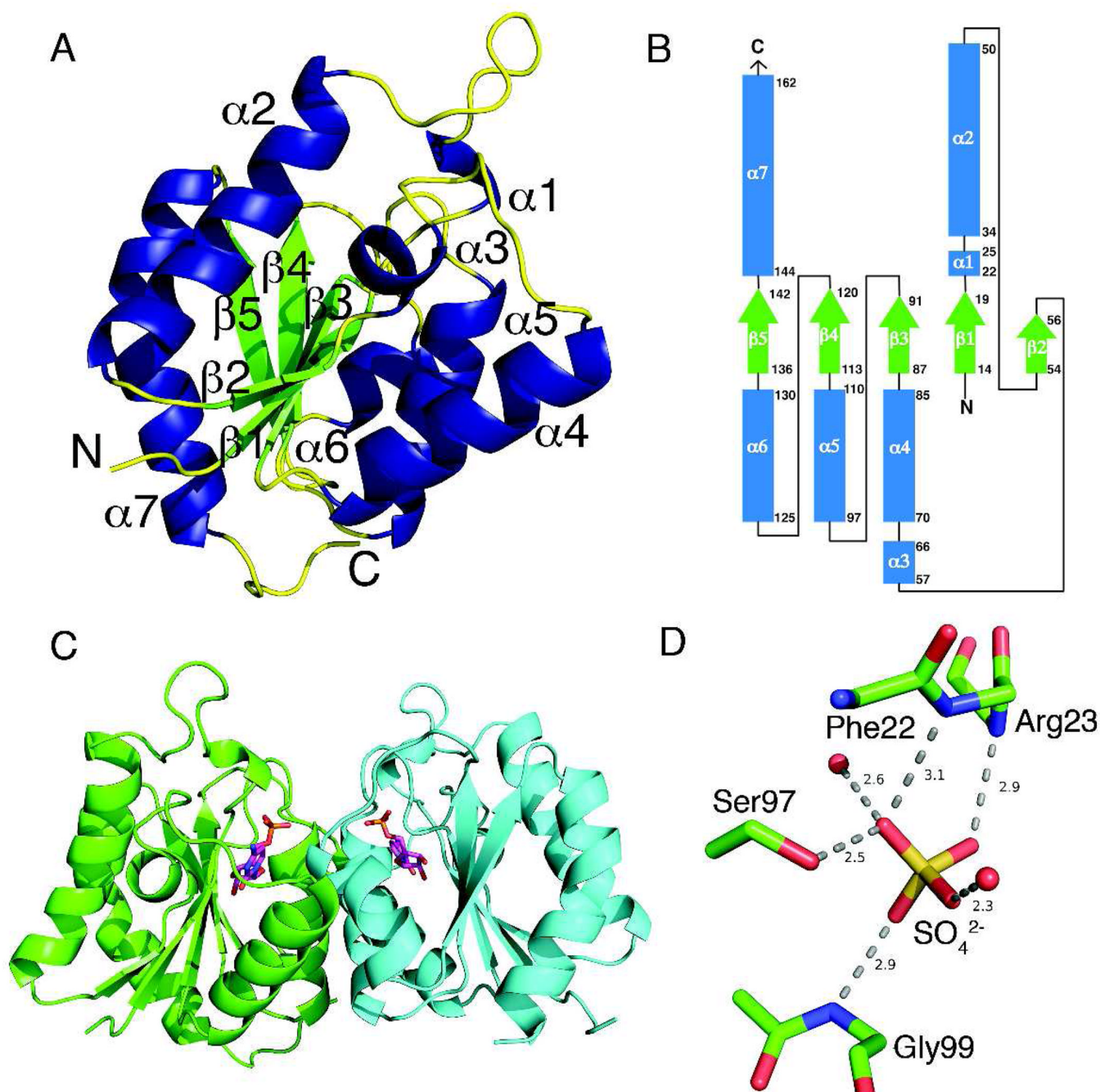
Figure 2. Structure of MilB. (A) The MilB protomer structure adopts an overall \alpha/\beta -twist fold, depicted with \beta -strands in green and \alpha -helices in blue. (B) The topology diagram of MilB with \beta -strands in light green and \alpha -helices in light blue. (C) The dimeric structure of MilB with chain A in green and chain B in cyan and ligands bound in the active sites. (D) The active site phosphate-binding pocket is occupied by a sulfate ion in the MilB/SO 4 complex. The sulfate binding site corresponds to the phosphate binding site in the CMP complex.
