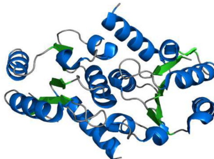
Rcl PDB: 4FYI
