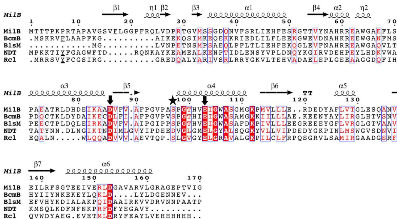
Figure 7. Sequence alignment of enzymes containing the nucleoside 2'-deoxyribosyltransferase motif. Sequence comparison between MilB/BcmB and other family members reveals conservation of the key catalytic residues (arrows) but not of those conferring substrate-binding specificity. The serine residue involved in phosphate binding is indicated with a star. Phenylalanine and tyrosine residues known to be positioned in the active site are underlined. Representative sequences for NDT from L. leichmannii and Rcl from R. norvegicus were used.
