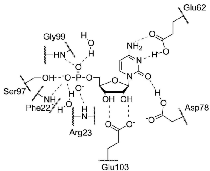
Figure 3. Substrate binding in MilB. (A) MilB-CMP binding interactions represented in stick view. (B) Schematic diagram of the MilB active site with CMP bound.
