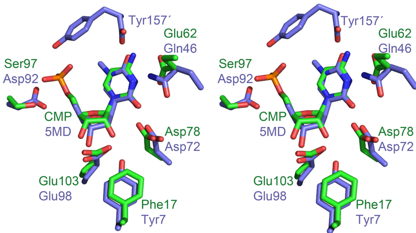
Figure 9. Active site comparison of MilB and NDT. A stereoview active site comparison between MilB with CMP bound (green) and NDT with 5-methyl-2'-deoxypseudouridine (5MD) (blue) reveals conserved positioning of the catalytic glutamate and aspartate residues. Other key residues for substrate binding deviate between the two structures.
