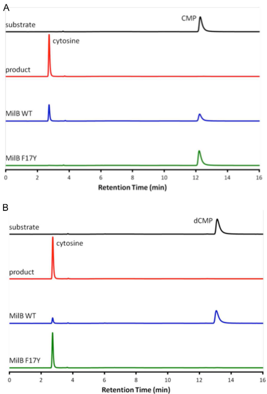
Figure 5. Substrate specificity of MilB WT and MilB F17Y. (A) When MilB WT is incubated with CMP a large peak representing free cytosine is observed. For MilB F17Y incubated with CMP, little hydrolysis is observed. (B) The opposite effect is observed with dCMP as substrate. MilB F17Y hydrolyzes dCMP producing free cytosine. There is comparably less dCMP hydrolysis by MilB WT.
