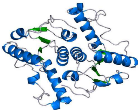
NDT PDB: 1F8X
