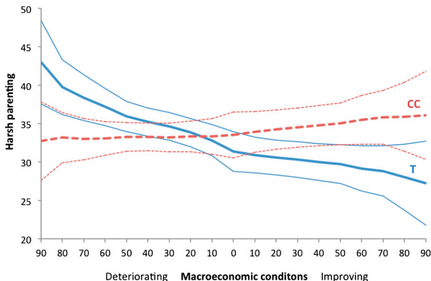
Fig. 1. Differential harsh parenting responses to deteriorating and improving macroeconomic conditions (measured as percentile changes) by the DRD2 Taq1A polymorphism.
