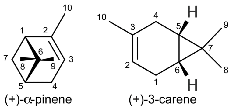
Figure 1. Molecular representations of (+)- \alpha -pinene and (+)-3-carene.
