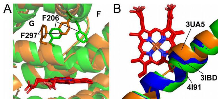
Figure 4. Structural differences revealed upon comparison of 2B6 (+)- \alpha -pinene complex and amlodipine complex. A) Active site of 2B6 (+)- \alpha -pinene (orange) and 2B6 amlodipine (green) complex structures. B) Rearrangement of the I-helix among the 2B6 amlodipine (3UA5, orange), 4-CPI (3IBD, blue), and (+)- \alpha -pinene (4I91, green) complexes.
