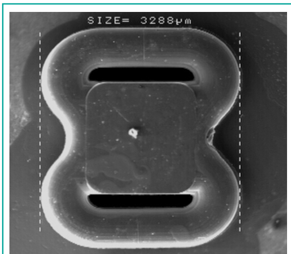
Figure 3 SEM micrograph of a not-used grey polyurethane Slide low-friction ligatures (GS) at original magnification x20.
