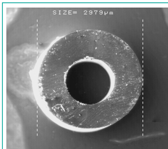
Figure 1 SEM micrograph of a not-used transparent elastomeric ligatures of ring type in latex (TR) at original magnification x20.
