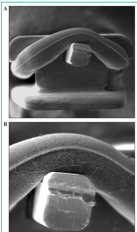
Figure 10 SEM micrograph of the interface between bracket, orthodontic arch and grey ligatures of ring type in polyurethane (GR) after 4 weeks of permanence in oral cavity at original magnification x30 (A) and x75 (B).
