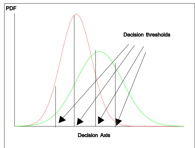
Figure 1. The two overlapping distributions (binormal model: probability density function-PDF) for diseased (right side) and nondiseased (left side) and four different decision threshold
