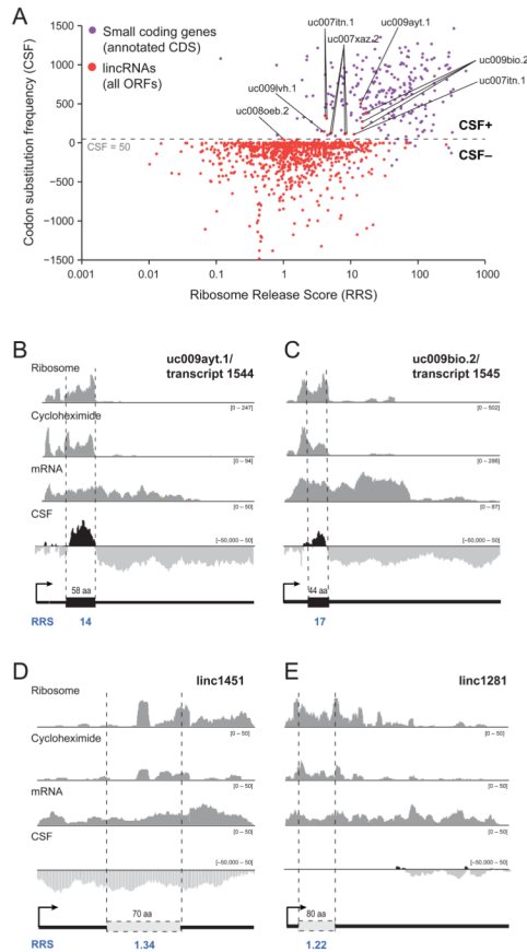
Figure 4. Ribosome release separates lincRNAs from small coding genes (a) A scatter plot of the RRS (log scale, x-axis) versus the CSF (y-axis) is plotted for each ORF of the lincRNAs (red points) and known small peptides (purple points). The dashed line corresponds to a CSF score of 50, the cutoff used to define a CSF+ set (CSF \geq 50) and CSF- set (CSF < 50) (see Methods ). (b) An example of a representative CSF+ transcript encoding a likely 58 amino acid protein with an RRS of 14. The four rows (ribosome, cycloheximide, mRNA and CSF) are as described in legend of Figure 1. The RRS score is noted in blue beneath the ideogram. (c) Another representative CSF+ transcript encoding a likely 44 amino acid protein with an RRS of 17. (d) A representative CSF- transcript, linc1451. The putative ORF (white) is defined as the ORF with the highest ribosome occupancy and has an RRS of 1.34. (e) Another representative CSF- transcript, linc1281. The putative ORF (white) has an RRS of 1.22. See also Figure S4.
