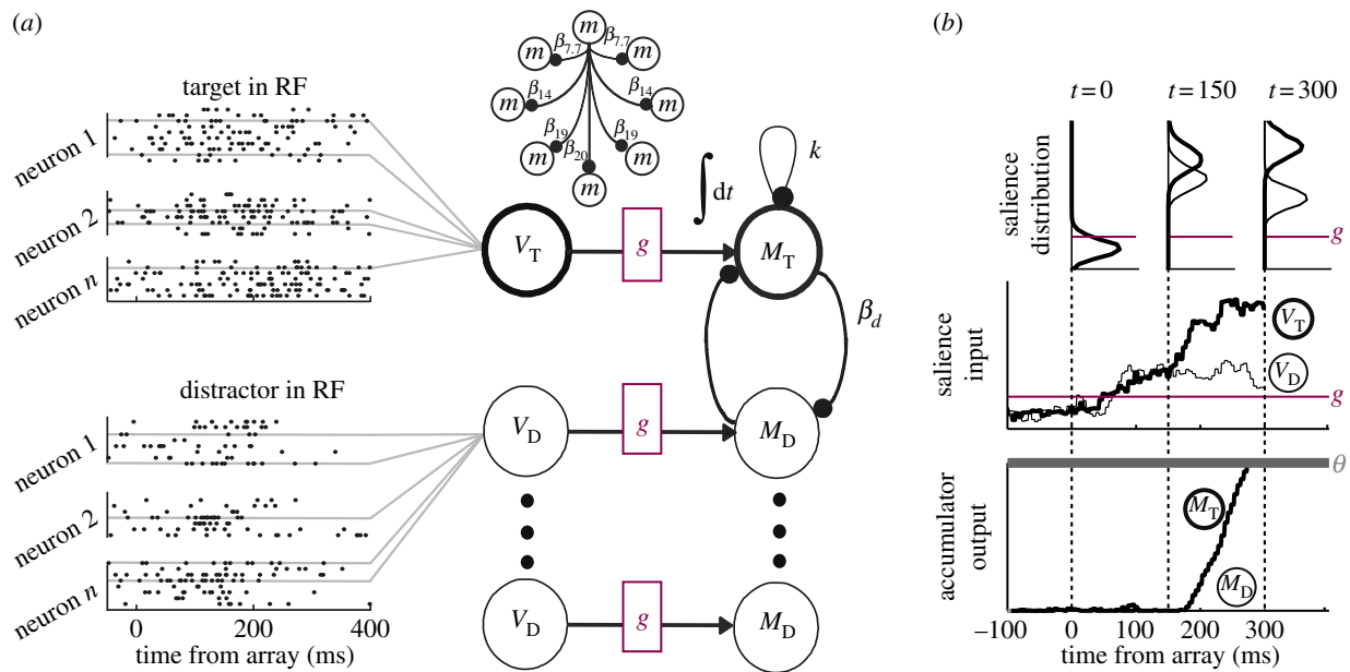
Figure 3. Gated stochastic accumulator model. (a) Neural activity recorded from FEF visual neurons provided saliency input. V_T , activity when a target fell in the neuron's RF, V_D , activity when distractors fell in the RF. Saliency input was gated, g such that stochastic accumulation could not begin until a critical level of input was achieved. Once reached, movement units corresponding to choices into ( M_T ) or away from ( M_D ) the RF began accumulating evidence. Movement accumulators were subject to leakage, k and lateral inhibition, \beta_d . (b) A decision was committed once accumulation reached a fixed threshold, \theta . The model not only accounts for overt behaviour but also accounts for the form of FEF movement neuron activity.
