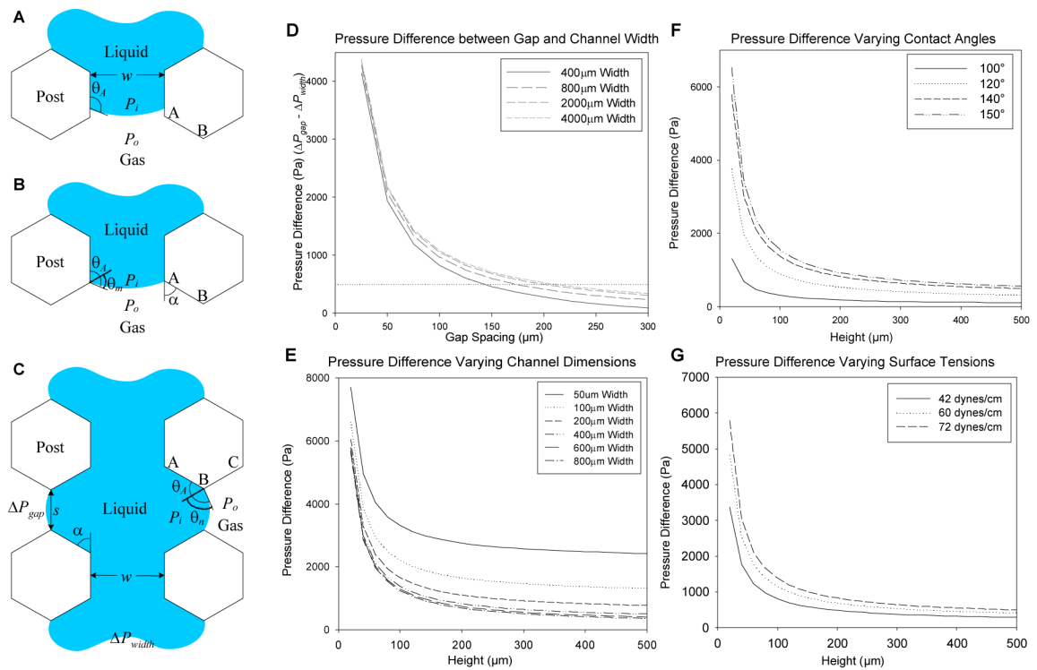
Figure 2. (A–C) Diagram of a filling process within a channel. During injection, a difference in pressure occurs at the air-liquid interface ( \Delta P ) which depends on surface tension forces ( \gamma ), channel geometry ( w and s ), and contact angles with the wall of the advancing liquid ( \theta_A ). (B) When the liquid interface encounters a gap spacing (point AB), a new contact angle ( \theta_m ) develops. (C) The difference between the gap spacing ( \Delta P_{gap} ) and channel ( \Delta P_{width} ) need to be maximized to prevent gel leakage. (D–G) Graphs of calculated pressure differences across a variety of parameters: height (E–F), width (E), contact angles (F), and surface tension (G). (D) Graph of pressure differences of increasing gap spacing. A threshold of 500 Pa was set empirically for criteria to prevent leakages and drawn as a guide for reference.
