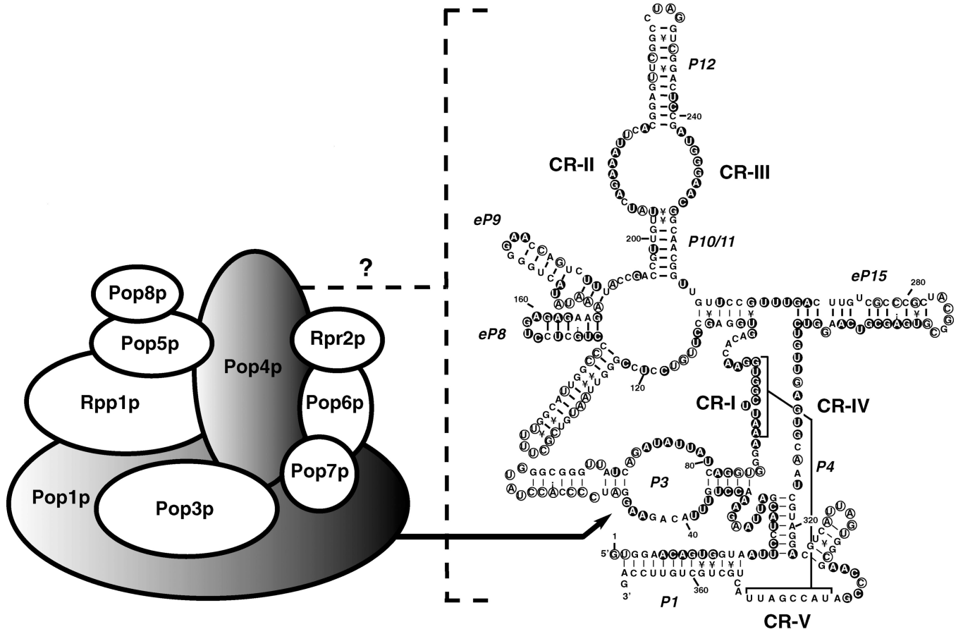
Figure 1. Summary of the yeast two-hybrid and three-hybrid test results of yeast ( S. cerevisiae ) nuclear RNase P. Ovals represent the protein subunits of yeast nuclear RNase P (Table 1). Overlaps of the ovals indicate a positive result in the two-hybrid test (141a). The shaded ovals of Pop1p and Pop4p indicate that they are the only protein subunits that interact specifically with the RPR1 RNA in a three-hybrid test. One of the recognition sites in the RPR1 RNA for Pop1p binding is the P3 loop, as indicated by the arrow (116). The binding sites for Pop4p are currently unknown, which is represented by the dotted bracket and a question mark. The predicted secondary structure of RPR1 RNA is adapted from the model proposed by Frank et al (15). Five critical regions, CR-I to CR-V, are numbered based on the Chen & Pace nomenclature (14). P represents helical regions, with numbers assigned according to the bacterial structure (101). eP indicates the eukaryotic paired regions whose homology to particular bacterial structures is uncertain, but which occupy the same positions as in the bacterial structure (15). Nucleotides in filled circles show protection from chemical modification and nuclease attack in the holoenzyme, whereas the nucleotides in open circles indicate exposure to solution (16).
