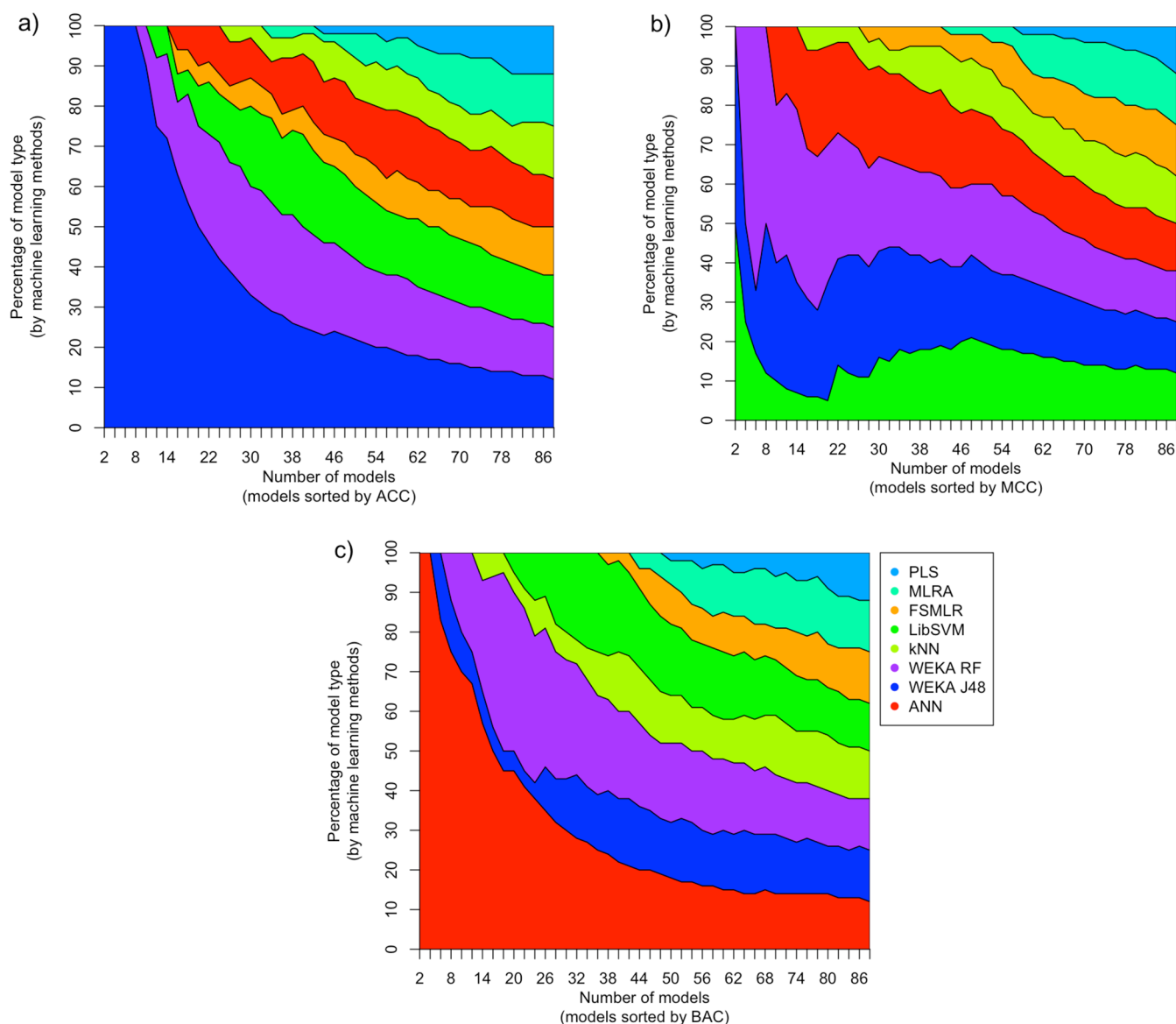
Figure 2. Percentage of models contributed by different methods (y-axis) as a function of the number of n top-ranked models ( x -axis) selected according to accuracy (ACC), Mathew correlation coefficient (MCC), and balanced accuracy (BAC).
