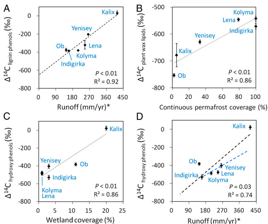
Fig. 3. Hydrological and physiogeographic controls on the age of terrestrial markers in the integrating Eurasian Arctic estuaries: correlation of \Delta^{14}\text{C}_{\text{lignin phenols}} with runoff rate (A), \Delta^{14}\text{C}_{\text{plant wax lipids}} with continuous permafrost coverage (B), \Delta^{14}\text{C}_{\text{hydroxy phenols}} with wetland coverage (C), and \Delta^{14}\text{C}_{\text{hydroxy phenols}} with runoff rate (D). The blue dotted line in D represents linear correlation for the data of four eastern rivers ( P < 0.05 , R^2 = 0.81 ). *Runoff rate = discharge/basin area. Contents of terrestrial markers are defined in Fig. 2. Further statistical analyses can be found in Fig. S2.
