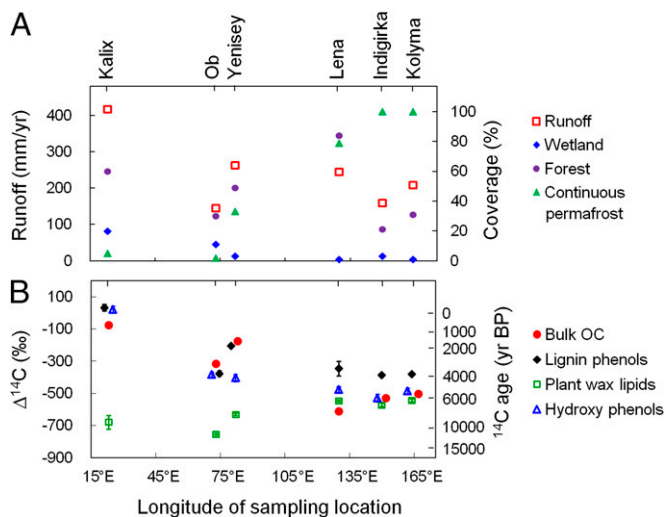
Fig. 2. Hydrogeographic characteristics of the Eurasian Arctic rivers (A) and contrasting radiocarbon contents (expressed as \Delta^{14}\text{C} and conventional ^{14}\text{C} age) of terrestrial markers compared with bulk OC in the estuarine surface sediments (B). Runoff rate = discharge/basin area. Detailed hydrogeographic data are listed in Table S1 [compiled from refs. 6, 9, 27, 52 and “watersheds of the world” ( http://www.wri.org/publications )]. The \Delta^{14}\text{C} values of terrestrial markers represent concentration-weighted averages with the SEs of analytical measurement propagated. Lignin phenols refer to vanillyl and syringyl phenols (detailed data are provided in Fig. S1). Hydroxy phenols refer to p -hydroxybenzaldehyde, p -hydroxyacetophenone, and p -hydroxybenzoic acid. Plant wax lipids constitute n -alkanes ( \text{C}_{27,29,31} ) and n -alkanoic acids ( \text{C}_{24,26,28} ) (6).
