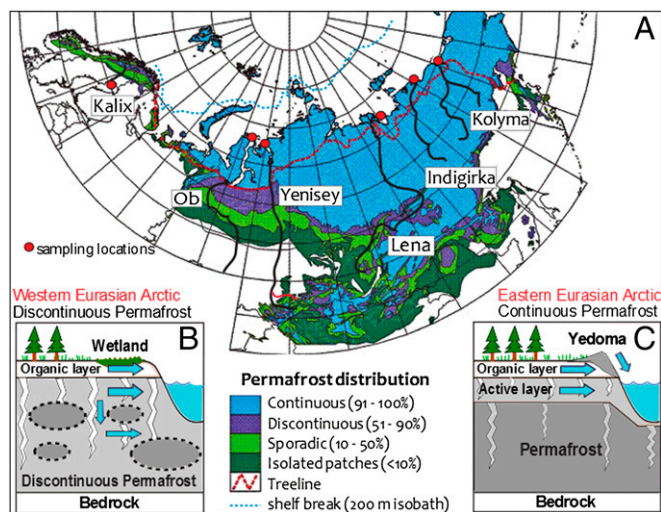
Fig. 1. Eurasian Arctic transect and cartoon of hydrological mobilization of terrestrial carbon into rivers. (A) Map of the rivers (black lines) with permafrost distribution (modified from refs. 1 and 6) and sampling locations (red circles). (B) Illustration of the western Eurasian Arctic characterized by extensive moss-dominated wetlands underlain by discontinuous permafrost and ubiquitous deep groundwater conduits. (C) Illustration of eastern Eurasian Arctic characterized by a wide distribution of Yedoma ice complex, a thin seasonally thawing active layer, and thick continuous permafrost below. Blue arrows indicate hydrological transport of carbon from different physiogeographic regimes.
