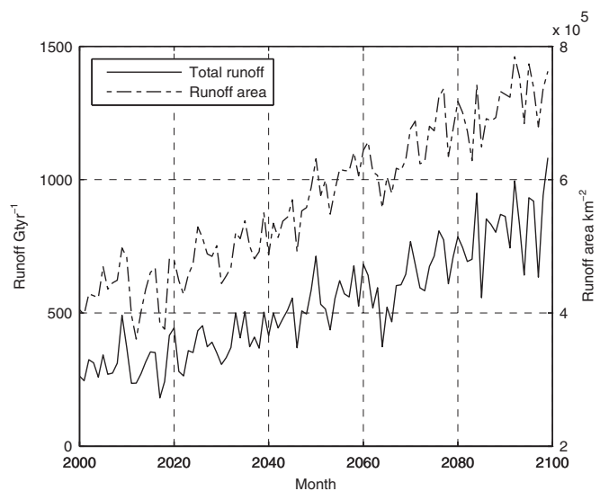
Fig. 1. Time series of the total runoff and runoff area for 2000–2100 simulated by the MAR. The runoff area is defined as areas with runoff greater than 1 \text{ cm} \cdot \text{yr}^{-1} .
