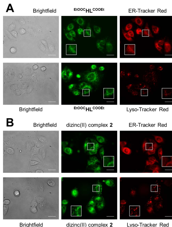
Figure 8. Fluorescence microscopy images of live SW480 cells. Cells were costained with 10 \mu\text{M} of \text{EtOOC-HL}^{\text{COOEt}} (A) or 5 \mu\text{M} of 2 (B) and ER-Tracker Red (500 nM) and Lyso-Tracker Red (1 \mu\text{M} ), respectively. Magnification of areas marked by squares are shown as insets. Scale bars are 20 \mu\text{m} .
