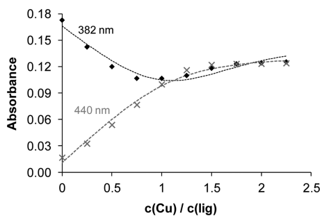
Figure 6. Measured and calculated (dashed lines) absorbance values at 382 nm ( \blacklozenge ) and 440 nm ( \times ) at various \text{EtOOC-HL-COOEt} -to-copper(II) ratios ( c_L = 10 \mu\text{M} ; c_{\text{Cu}} = 0\text{--}22.5 \mu\text{M} ; T = 298 \text{ K} ; l = 1 \text{ cm} , methanol).
