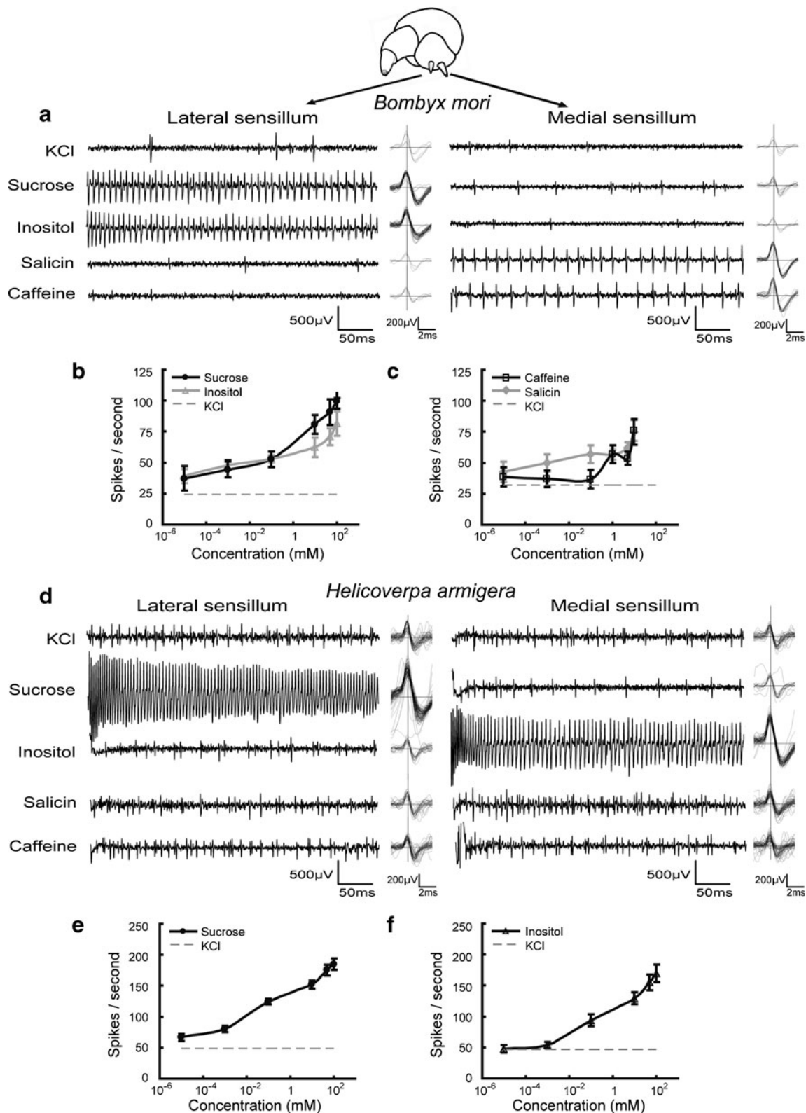
Fig. 5 Electrophysiological responses of Bombyx mori and Helicoverpa armigera larval gustatory receptor neurons (GRNs) to bitter and sweet stimuli. a Examples of spike traces from B. mori styloconic sensilla over the first 500 ms of stimulation, with spike shape superimposition. b, c Concentration-dependence of GRN responses to sucrose and myo -inositol in the lateral styloconic sensillum ( N=13 ) and to salicin and caffeine in the medial styloconic sensillum ( N=10 ). d Examples of spike traces from H. armigera
