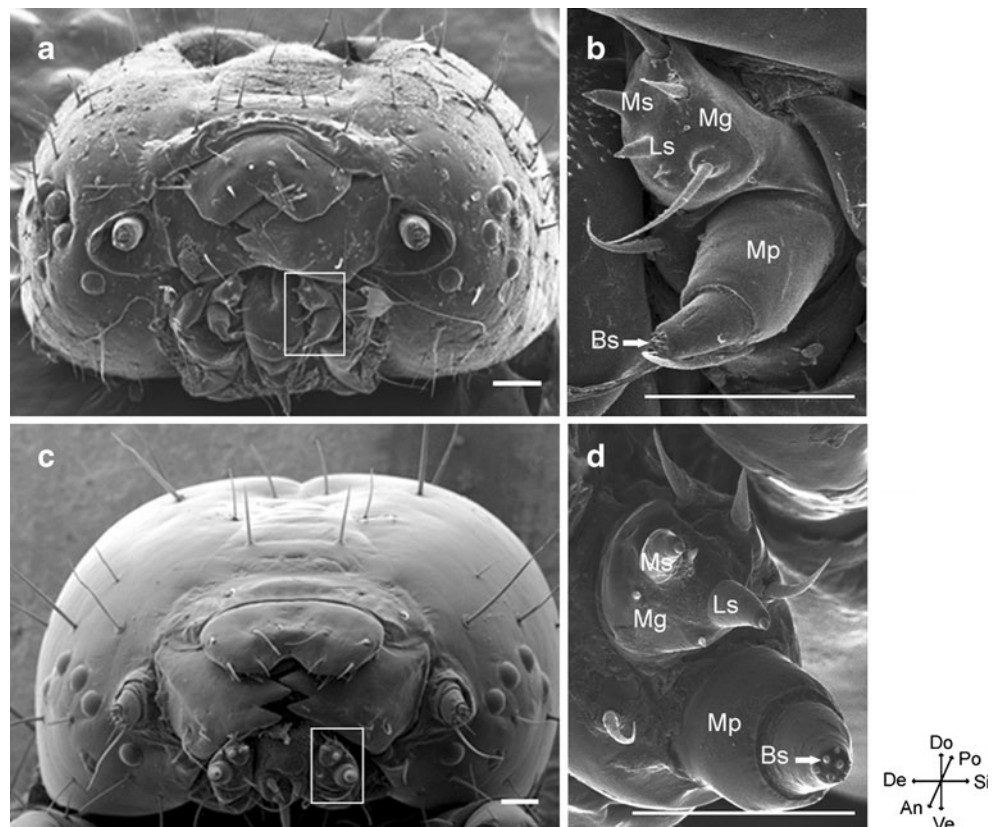
Fig. 3 Scanning electron micrographs of fifth instar heads showing maxillae. a, c Anterior images of Bombyx mori ( a ) and Helicoverpa armigera ( c ) heads. b, d Enlarged views of a maxilla of B. mori ( b ) and H. armigera ( d ). White rectangles indicate the location of maxillae. Mg, maxillary galea; Ms, medial styloconic sensillum; Ls, lateral styloconic sensillum; Mp, maxillary palp; Bs, basiconic sensillum. Do, dorsal; Po, posterior; Si, sinistral; Ve, ventral; An, anterior; De, dextral. Scale bar: 100 \mu m
