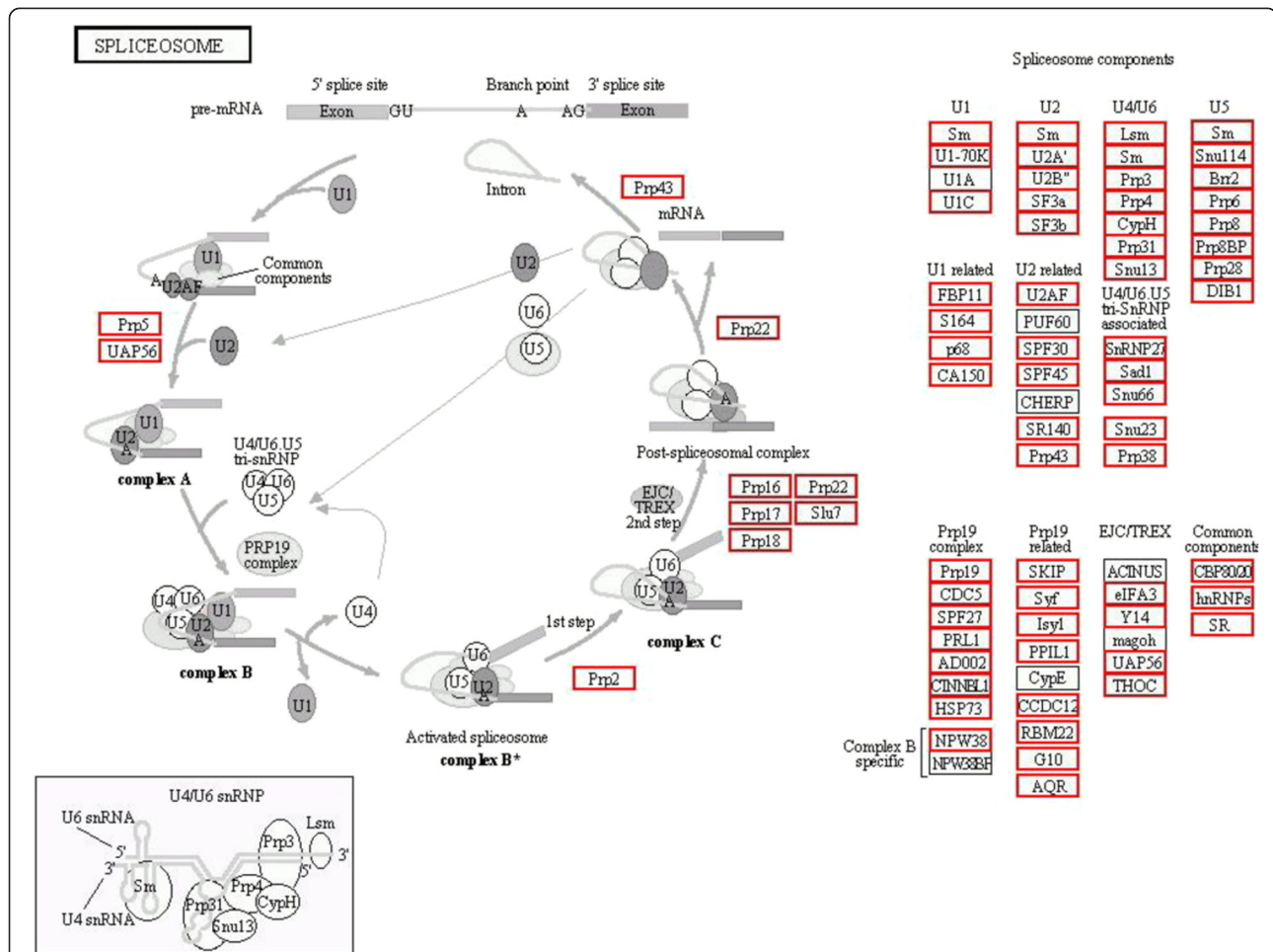
Figure 5 Spliceosome. 839(4.85%) unigenes were assigned to Spliceosome pathway by KEGG. The longan unigenes involving in the pathways are in red boxes.
