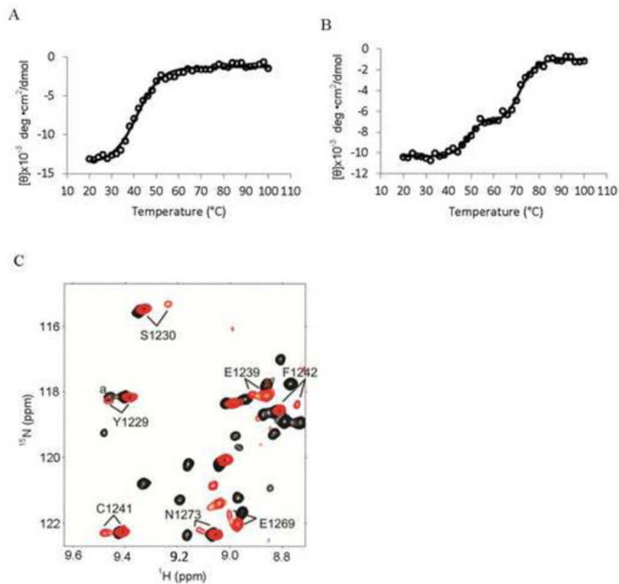
Fig. 2. The BRD and the CH2 domain are more stable in BRD-CH2 than the isolated domains. Thermal denaturation of the BRD (A) and BRD-CH2 (B) measured by CD spectroscopy. The CD values measured at 208 nm are plotted against temperature ranging from 20°C to 100°C. Open circles are raw data while the solid lines show the fitted values using a sigmoidal curve. (C) An overlay of a selected region of the HSQC spectra of the isolated CH2 domain (red) and BRD-CH2 (black), showing residues observed as two peaks only in the spectrum of the CH2 domain. a This peak in BRD-CH2 is from N1163.
