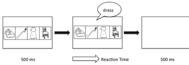
Fig. 2. Schematic of one trial of the SST
