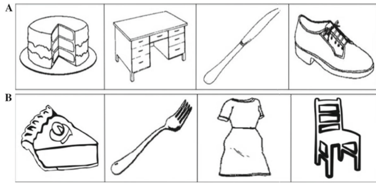
Fig. 1. Example of the visual display in Set A ( top ) and Set B ( bottom )
