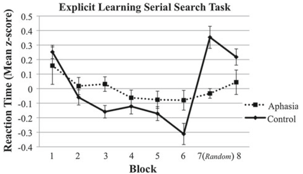
Fig. 4. Standardized reaction time values across the 8 blocks of the SST under explicit learning conditions in the aphasic and control groups. Bars represent one standard error above and below the mean
