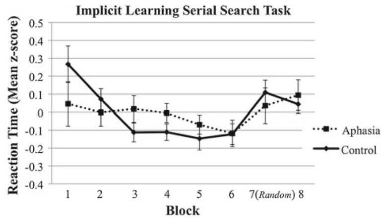
Fig. 3. Standardized reaction time values across the 8 blocks of the SST under implicit learning conditions in the aphasic and control groups. Bars represent one standard error above and below the mean
