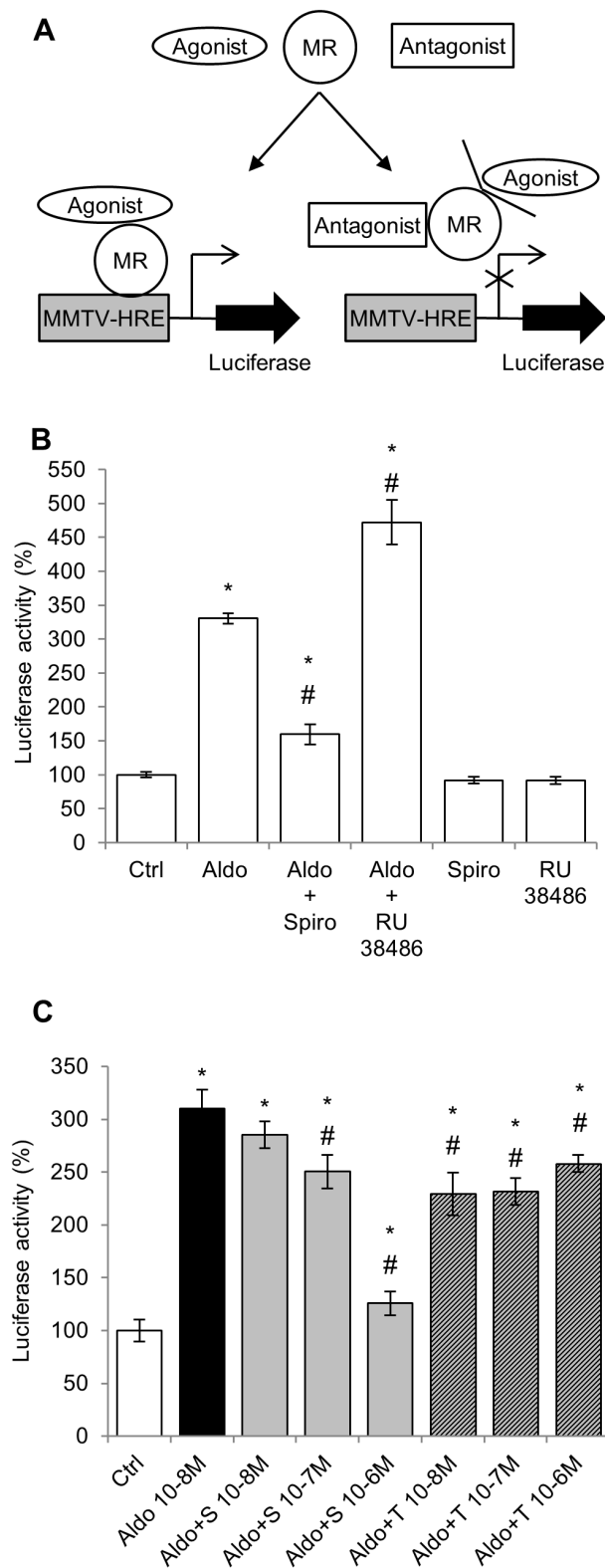
Figure 2. Effect of Torasemide on ligand-dependent transactivation activity of MR in H9C2-MR cells. A: The MMTV promoter contains Hormone Response Elements (HRE); the promoter sequence was fused to the Luciferase coding sequence. This construct was transfected into H9C2-MR cells. Upon binding of the aldosterone-MR complexes on HRE, luciferase is transcribed and light emission is enhanced, assessing MR transactivation activity. In the presence of an
